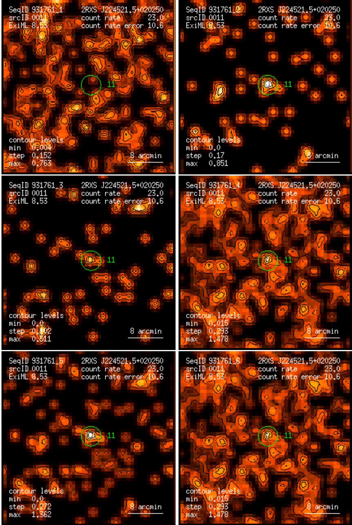
Figure 11: RASS 931761: detection 0011: band rate images, Gaussian filter: (1) PSPC channels 11 – 41, (2) 52 – 90, (3) 91 – 201, (4) 11 – 235, (5) 52 – 201, (6) 11 – 201. Broad band rates in counts/ks. Band rate contour levels in counts/ks/arcmin 2 .
