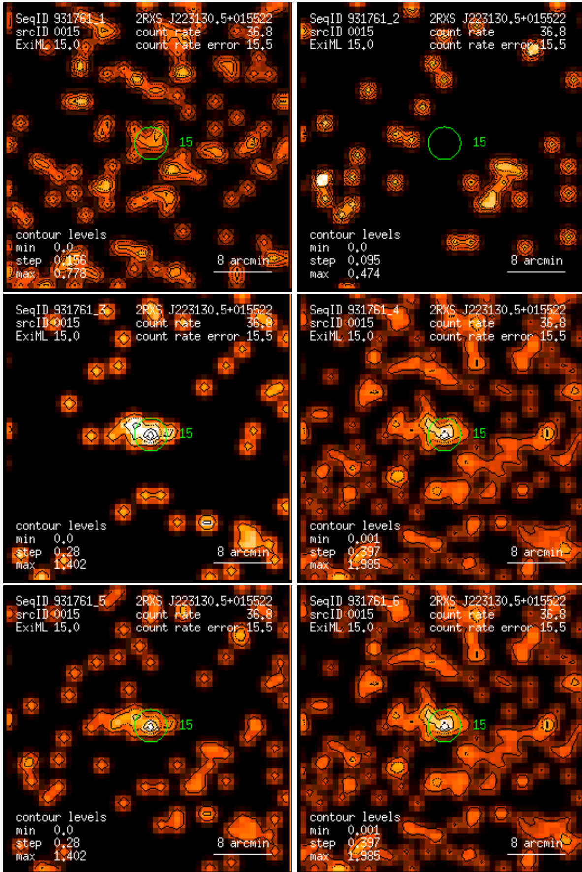
Figure 15: RASS 931761: detection 0015: band rate images, Gaussian filter: (1) PSPC channels 11 – 41, (2) 52 – 90, (3) 91 – 201, (4) 11 – 235, (5) 52 – 201, (6) 11 – 201. Broad band rates in counts/ks. Band rate contour levels in counts/ks/arcmin 2 .
