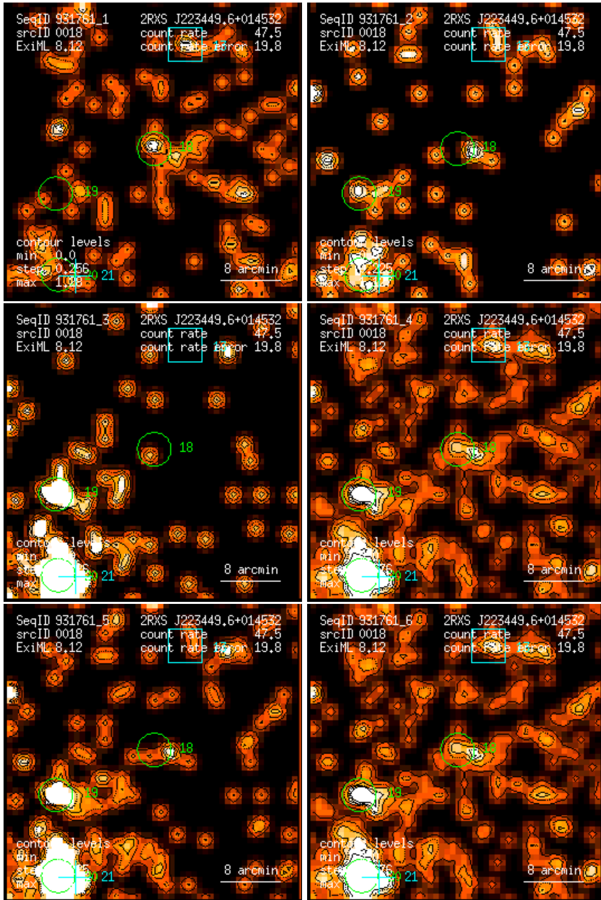
Figure 18: RASS 931761: detection 0018: band rate images, Gaussian filter: (1) PSPC channels 11 – 41, (2) 52 – 90, (3) 91 – 201, (4) 11 – 235, (5) 52 – 201, (6) 11 – 201. Broad band rates in counts/ks. Band rate contour levels in counts/ks/arcmin 2 .
