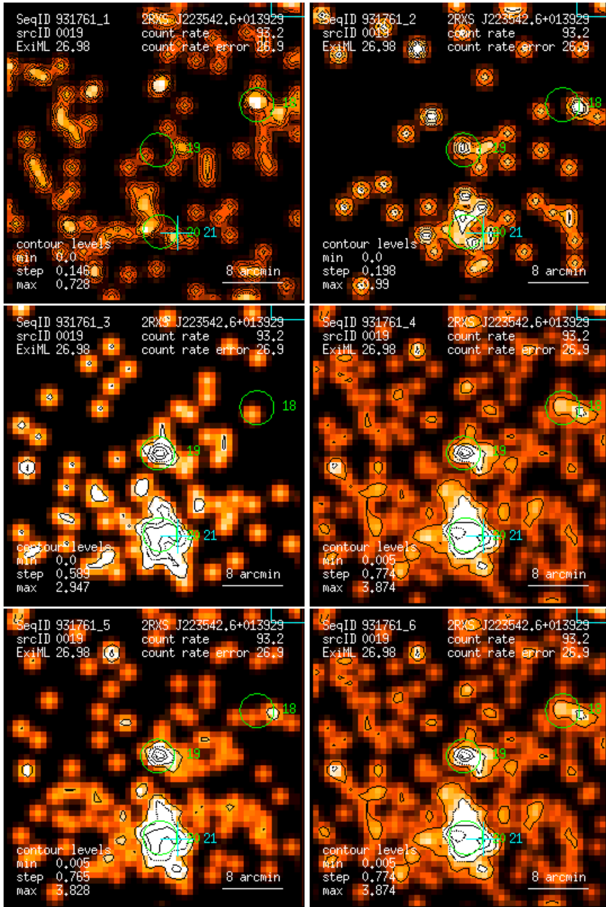
Figure 19: RASS 931761: detection 0019: band rate images, Gaussian filter: (1) PSPC channels 11 – 41, (2) 52 – 90, (3) 91 – 201, (4) 11 – 235, (5) 52 – 201, (6) 11 – 201. Broad band rates in counts/ks. Band rate contour levels in counts/ks/arcmin 2 .
