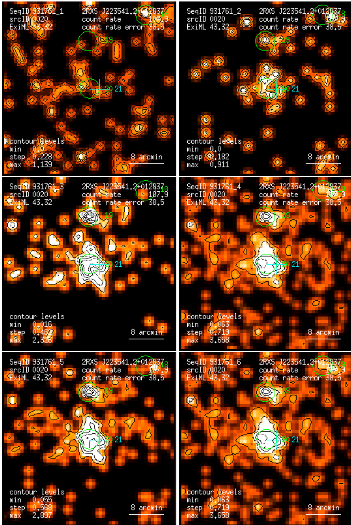
Figure 20: RASS 931761: detection 0020: band rate images, Gaussian filter: (1) PSPC channels 11 – 41, (2) 52 – 90, (3) 91 – 201, (4) 11 – 235, (5) 52 – 201, (6) 11 – 201. Broad band rates in counts/ks. Band rate contour levels in counts/ks/arcmin 2 .
