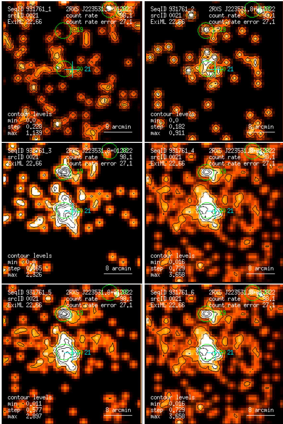
Figure 21: RASS 931761: detection 0021: band rate images, Gaussian filter: (1) PSPC channels 11 – 41, (2) 52 – 90, (3) 91 – 201, (4) 11 – 235, (5) 52 – 201, (6) 11 – 201. Broad band rates in counts/ks. Band rate contour levels in counts/ks/arcmin 2 .
