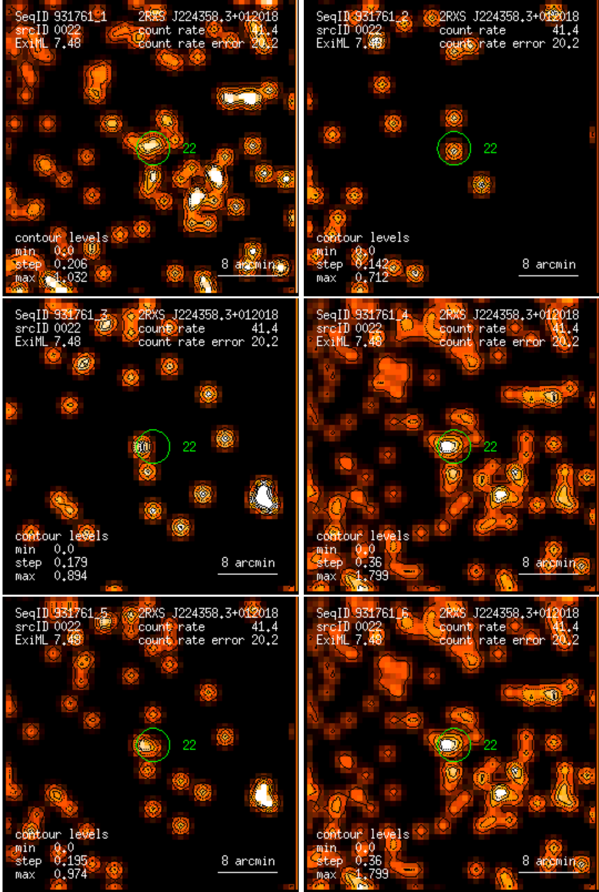
Figure 22: RASS 931761: detection 0022: band rate images, Gaussian filter: (1) PSPC channels 11 – 41, (2) 52 – 90, (3) 91 – 201, (4) 11 – 235, (5) 52 – 201, (6) 11 – 201. Broad band rates in counts/ks. Band rate contour levels in counts/ks/arcmin 2 .
