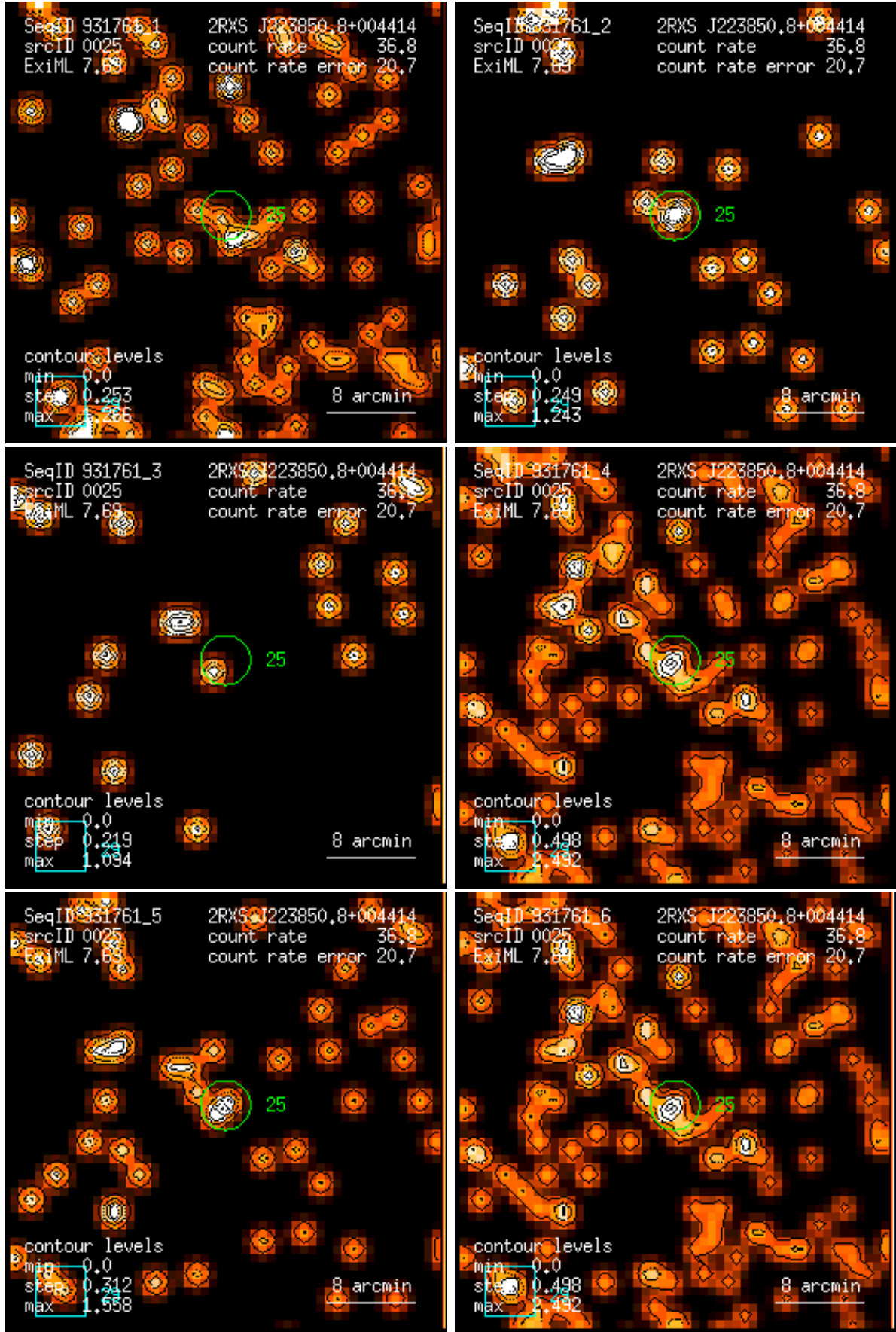
Figure 25: RASS 931761: detection 0025: band rate images, Gaussian filter: (1) PSPC channels 11 – 41, (2) 52 – 90, (3) 91 – 201, (4) 11 – 235, (5) 52 – 201, (6) 11 – 201. Broad band rates in counts/ks. Band rate contour levels in counts/ks/arcmin 2 .
