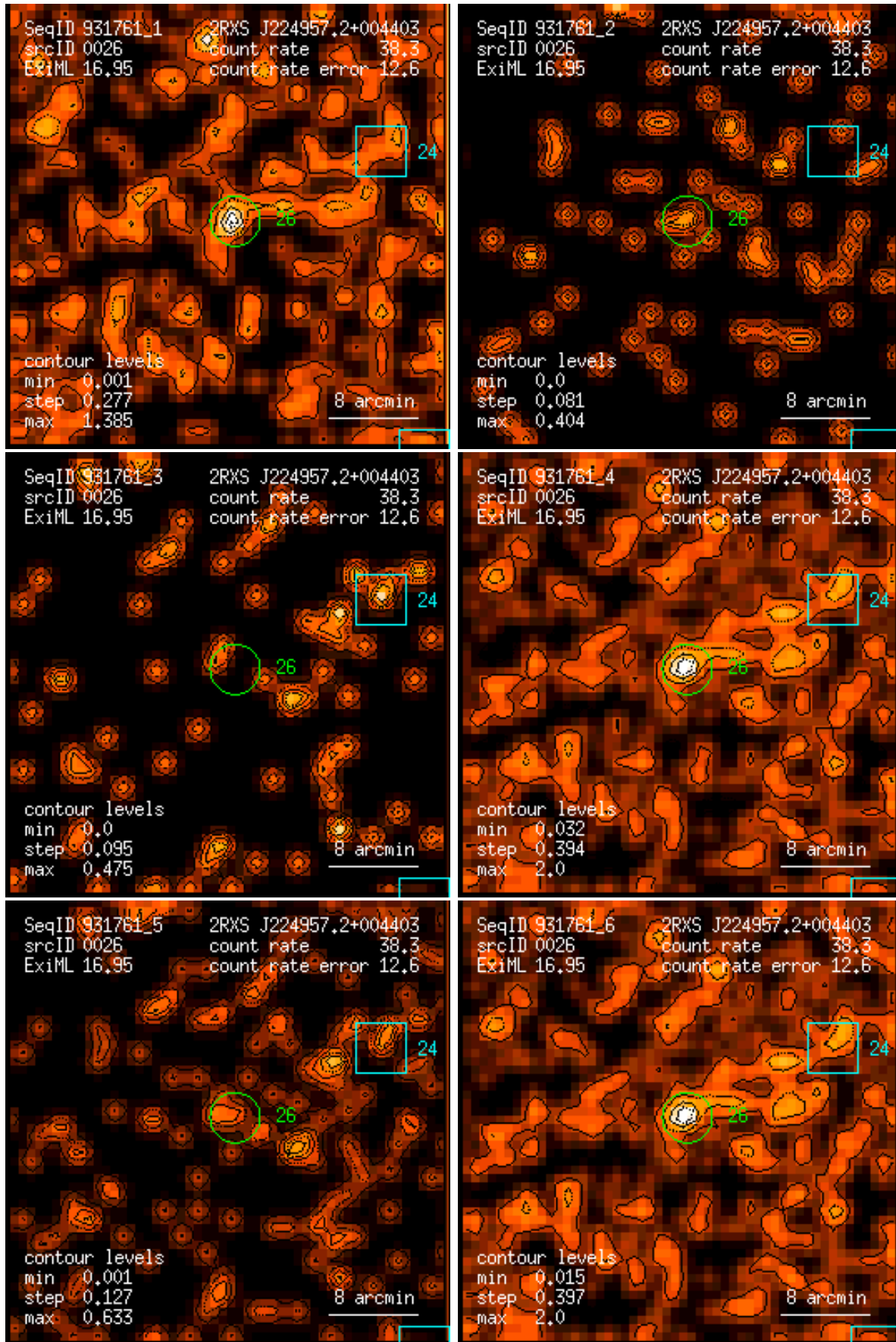
Figure 26: RASS 931761: detection 0026: band rate images, Gaussian filter: (1) PSPC channels 11 – 41, (2) 52 – 90, (3) 91 – 201, (4) 11 – 235, (5) 52 – 201, (6) 11 – 201. Broad band rates in counts/ks. Band rate contour levels in counts/ks/arcmin 2 .
