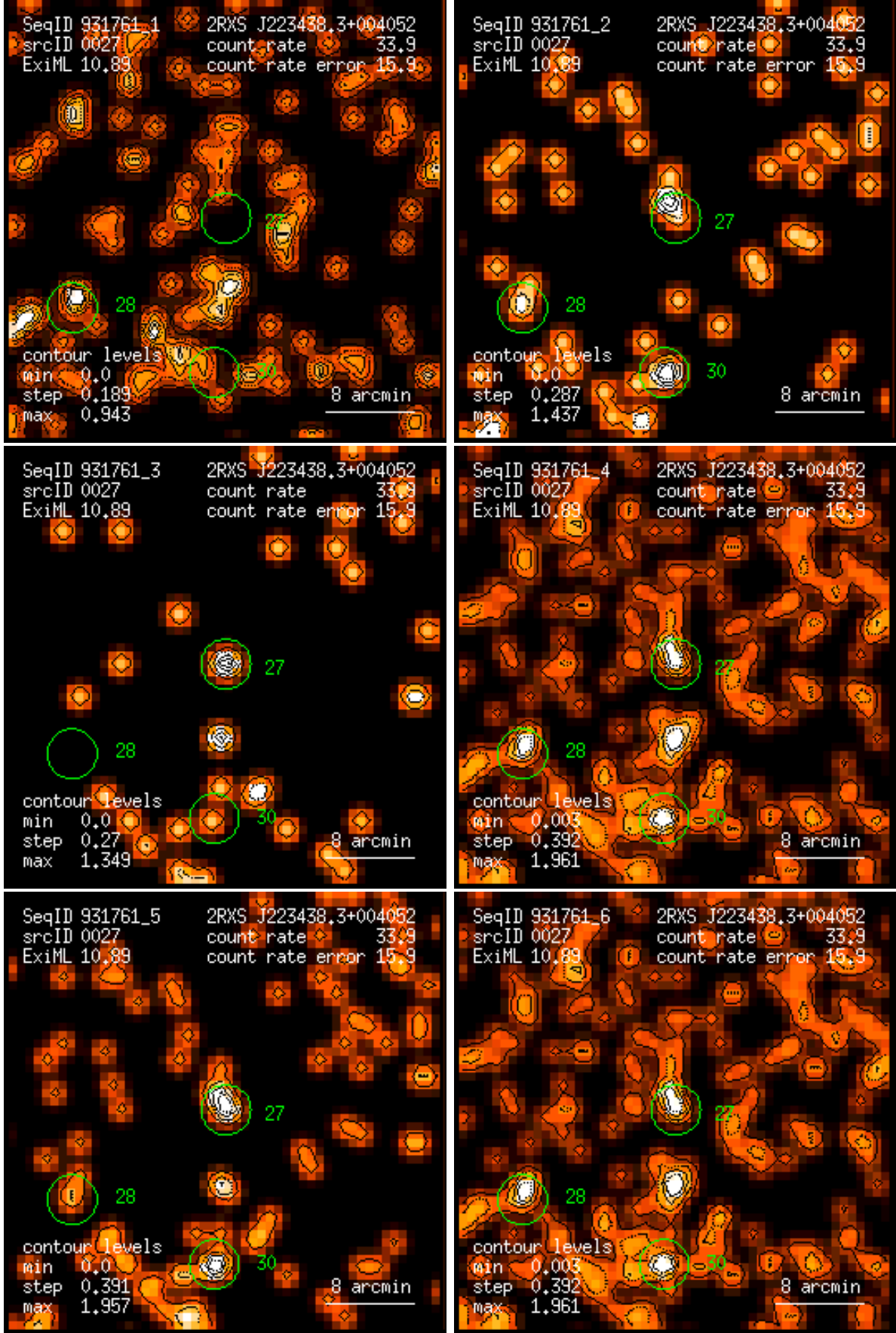
Figure 27: RASS 931761: detection 0027: band rate images, Gaussian filter: (1) PSPC channels 11 – 41, (2) 52 – 90, (3) 91 – 201, (4) 11 – 235, (5) 52 – 201, (6) 11 – 201. Broad band rates in counts/ks. Band rate contour levels in counts/ks/arcmin 2 .
