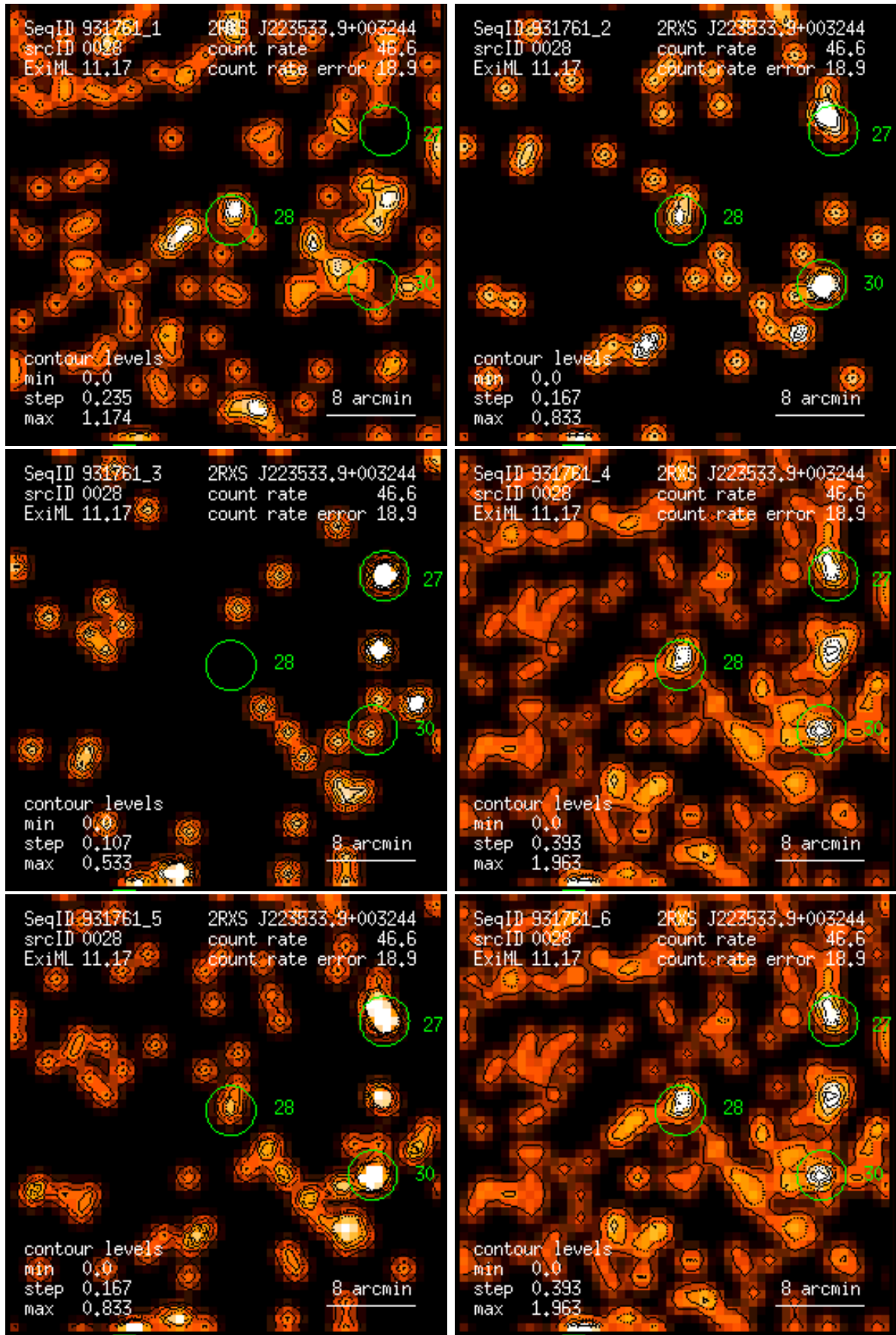
Figure 28: RASS 931761: detection 0028: band rate images, Gaussian filter: (1) PSPC channels 11 – 41, (2) 52 – 90, (3) 91 – 201, (4) 11 – 235, (5) 52 – 201, (6) 11 – 201. Broad band rates in counts/ks. Band rate contour levels in counts/ks/arcmin 2 .
