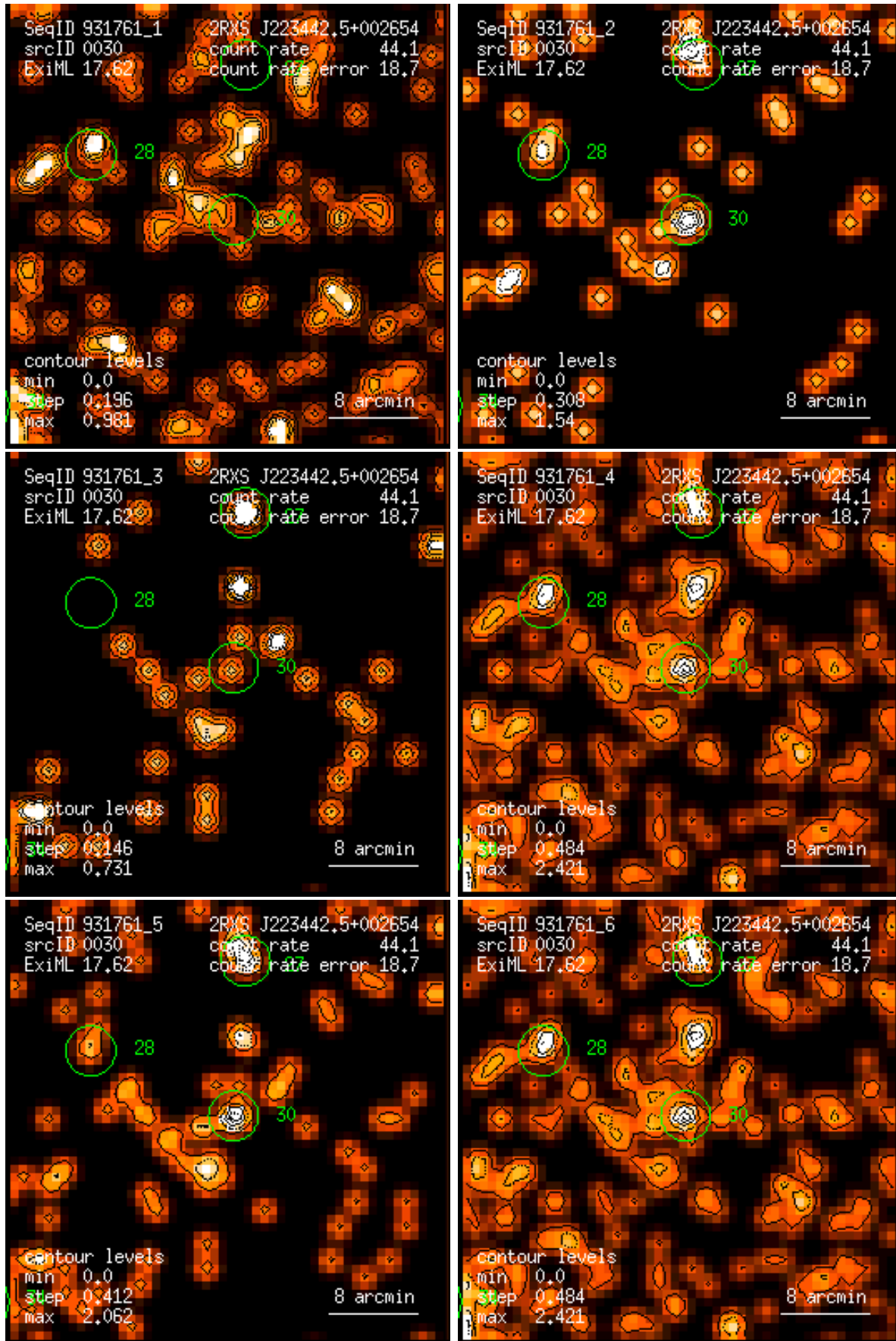
Figure 30: RASS 931761: detection 0030: band rate images, Gaussian filter: (1) PSPC channels 11 – 41, (2) 52 – 90, (3) 91 – 201, (4) 11 – 235, (5) 52 – 201, (6) 11 – 201. Broad band rates in counts/ks. Band rate contour levels in counts/ks/arcmin 2 .
