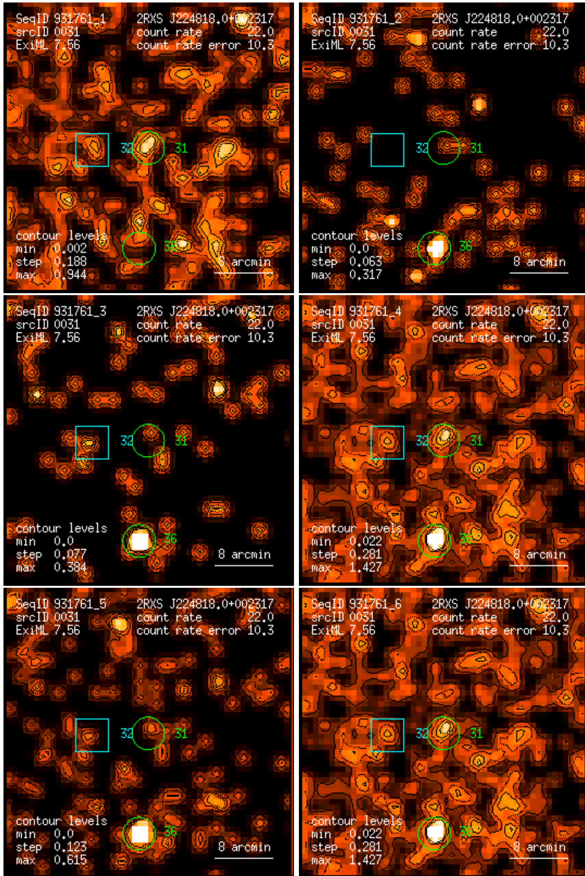
Figure 31: RASS 931761: detection 0031: band rate images, Gaussian filter: (1) PSPC channels 11 – 41, (2) 52 – 90, (3) 91 – 201, (4) 11 – 235, (5) 52 – 201, (6) 11 – 201. Broad band rates in counts/ks. Band rate contour levels in counts/ks/arcmin 2 .
