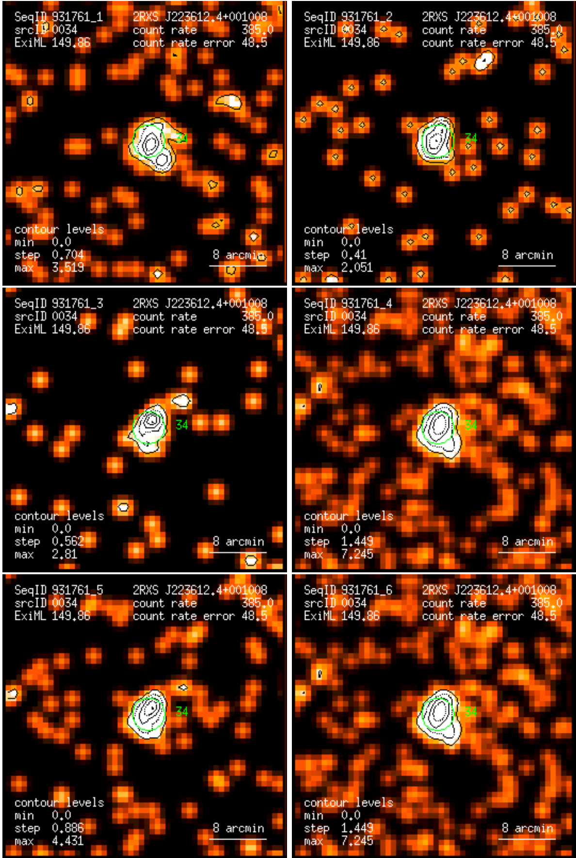
Figure 34: RASS 931761: detection 0034: band rate images, Gaussian filter: (1) PSPC channels 11 – 41, (2) 52 – 90, (3) 91 – 201, (4) 11 – 235, (5) 52 – 201, (6) 11 – 201. Broad band rates in counts/ks. Band rate contour levels in counts/ks/arcmin 2 .
