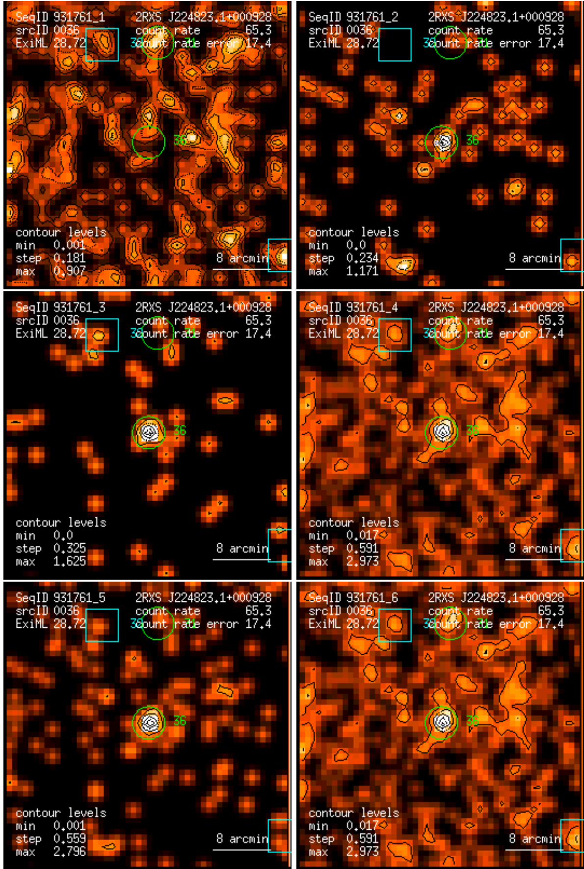
Figure 36: RASS 931761: detection 0036: band rate images, Gaussian filter: (1) PSPC channels 11 – 41, (2) 52 – 90, (3) 91 – 201, (4) 11 – 235, (5) 52 – 201, (6) 11 – 201. Broad band rates in counts/ks. Band rate contour levels in counts/ks/arcmin 2 .
