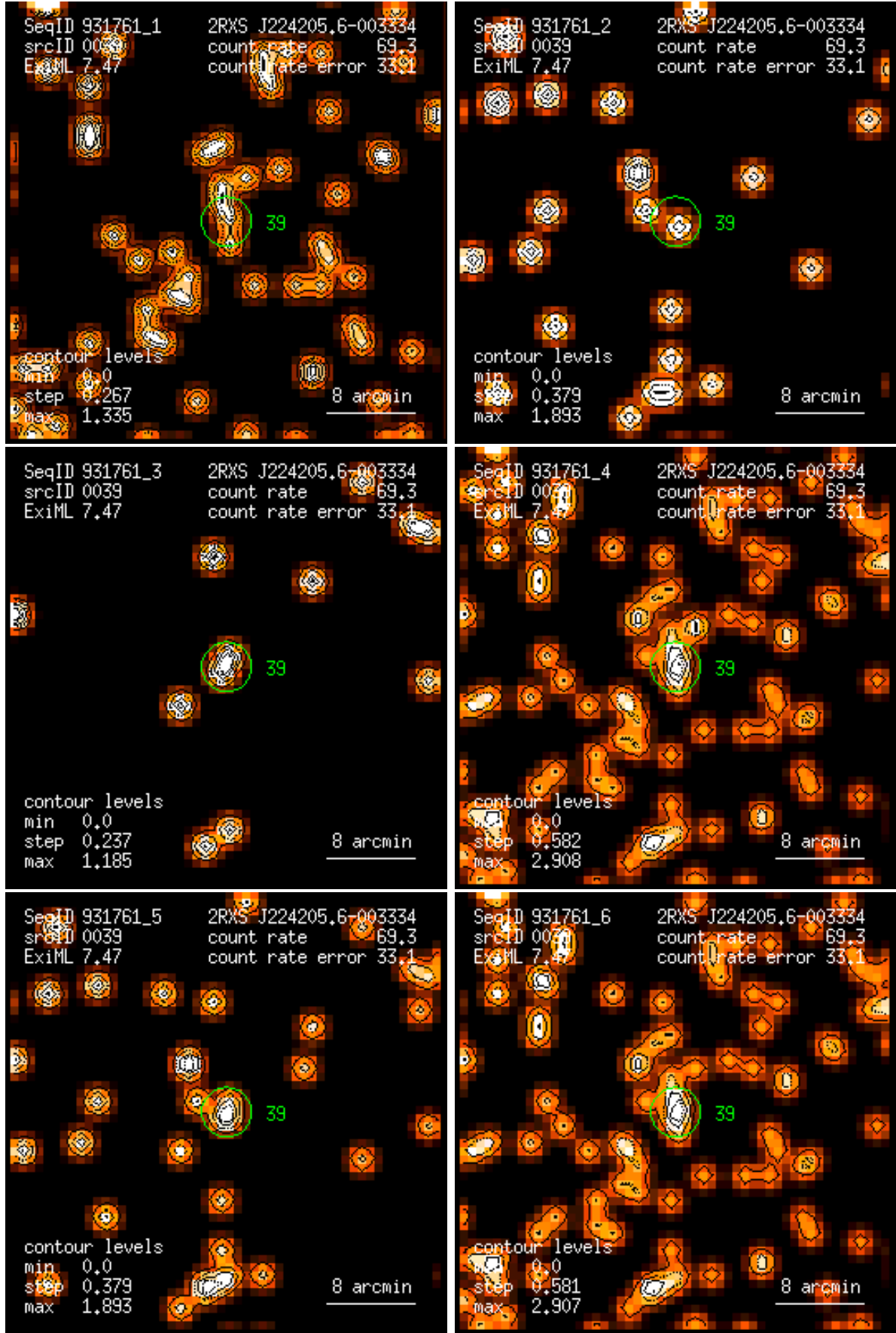
Figure 39: RASS 931761: detection 0039: band rate images, Gaussian filter: (1) PSPC channels 11 – 41, (2) 52 – 90, (3) 91 – 201, (4) 11 – 235, (5) 52 – 201, (6) 11 – 201. Broad band rates in counts/ks. Band rate contour levels in counts/ks/arcmin 2 .
