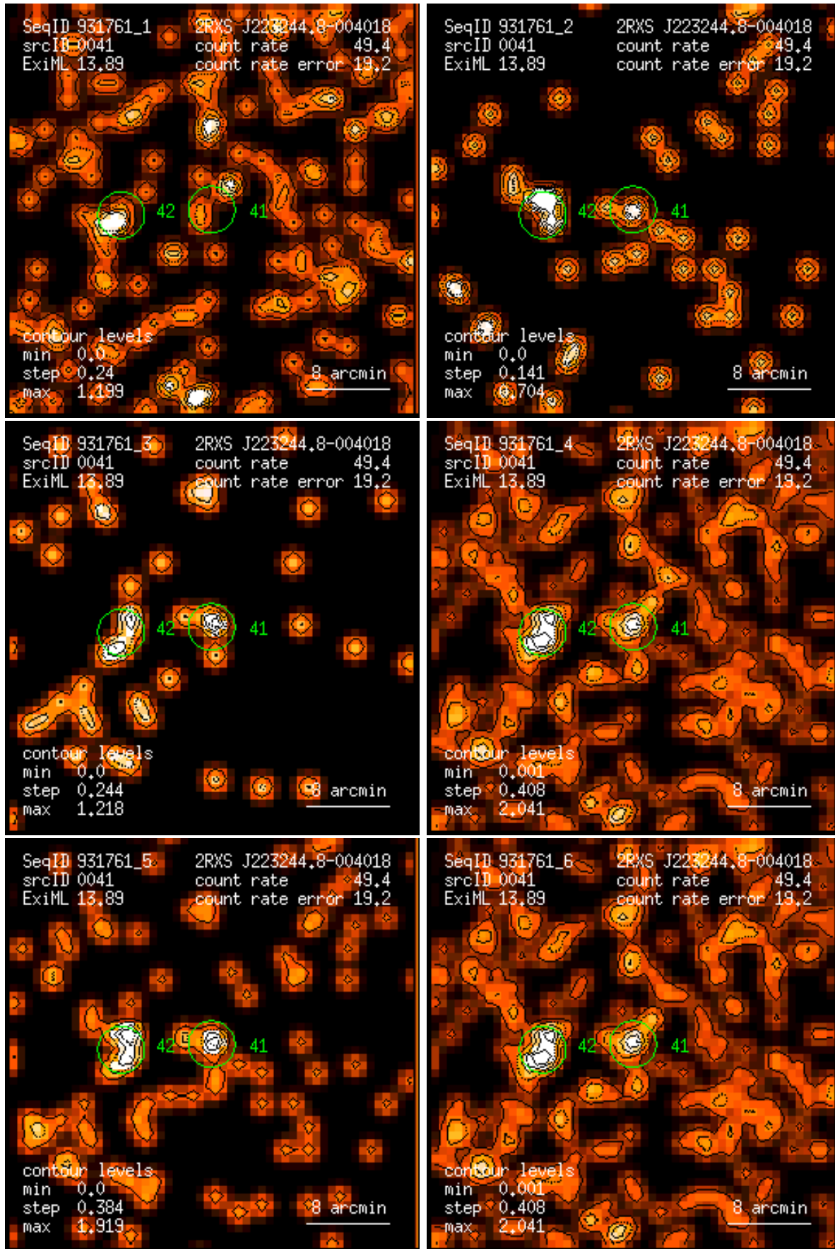
Figure 41: RASS 931761: detection 0041: band rate images, Gaussian filter: (1) PSPC channels 11 – 41, (2) 52 – 90, (3) 91 – 201, (4) 11 – 235, (5) 52 – 201, (6) 11 – 201. Broad band rates in counts/ks. Band rate contour levels in counts/ks/arcmin 2 .
