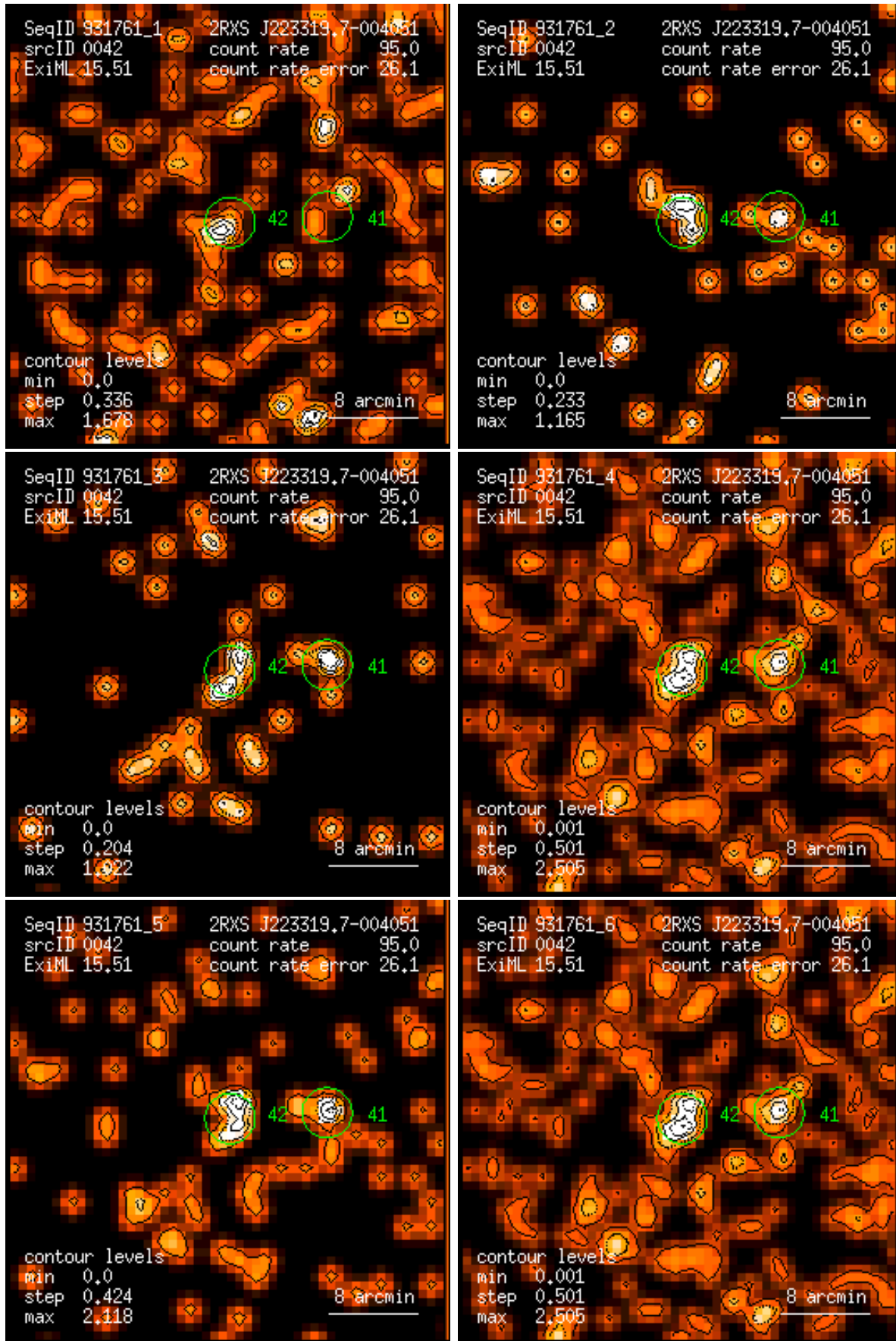
Figure 42: RASS 931761: detection 0042: band rate images, Gaussian filter: (1) PSPC channels 11 – 41, (2) 52 – 90, (3) 91 – 201, (4) 11 – 235, (5) 52 – 201, (6) 11 – 201. Broad band rates in counts/ks. Band rate contour levels in counts/ks/arcmin 2 .
