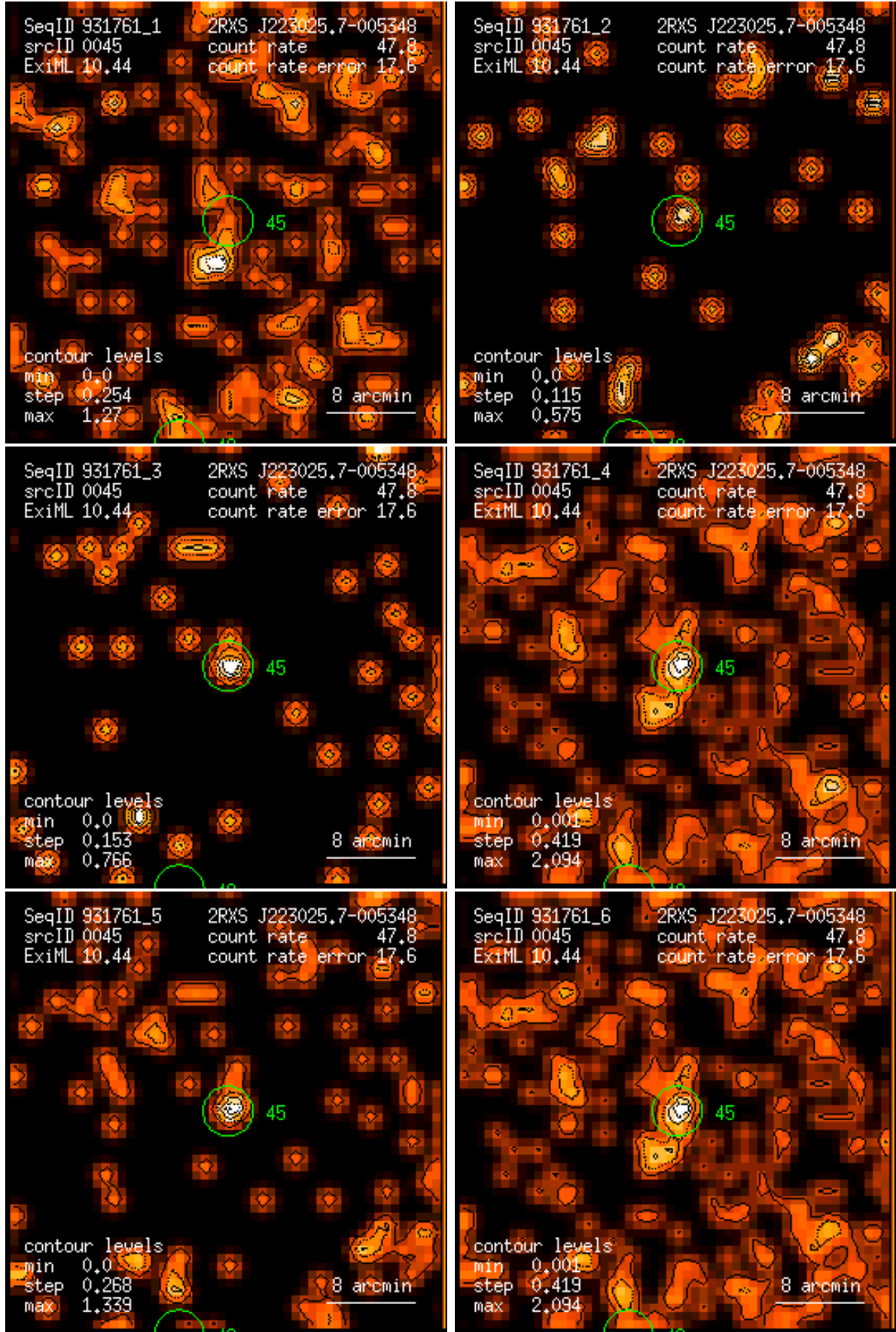
Figure 45: RASS 931761: detection 0045: band rate images, Gaussian filter: (1) PSPC channels 11 – 41, (2) 52 – 90, (3) 91 – 201, (4) 11 – 235, (5) 52 – 201, (6) 11 – 201. Broad band rates in counts/ks. Band rate contour levels in counts/ks/arcmin 2 .
