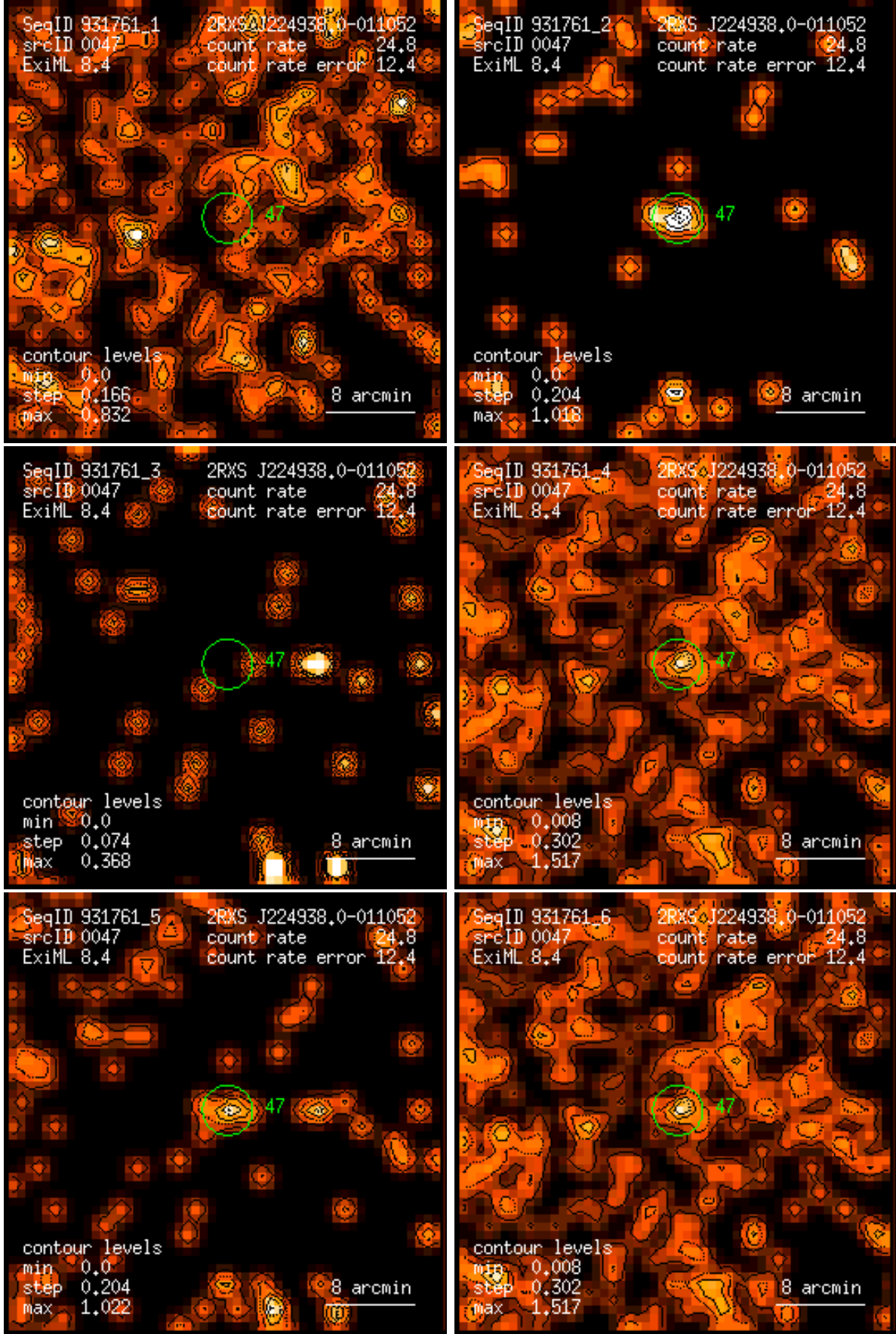
Figure 47: RASS 931761: detection 0047: band rate images, Gaussian filter: (1) PSPC channels 11 – 41, (2) 52 – 90, (3) 91 – 201, (4) 11 – 235, (5) 52 – 201, (6) 11 – 201. Broad band rates in counts/ks. Band rate contour levels in counts/ks/arcmin 2 .
