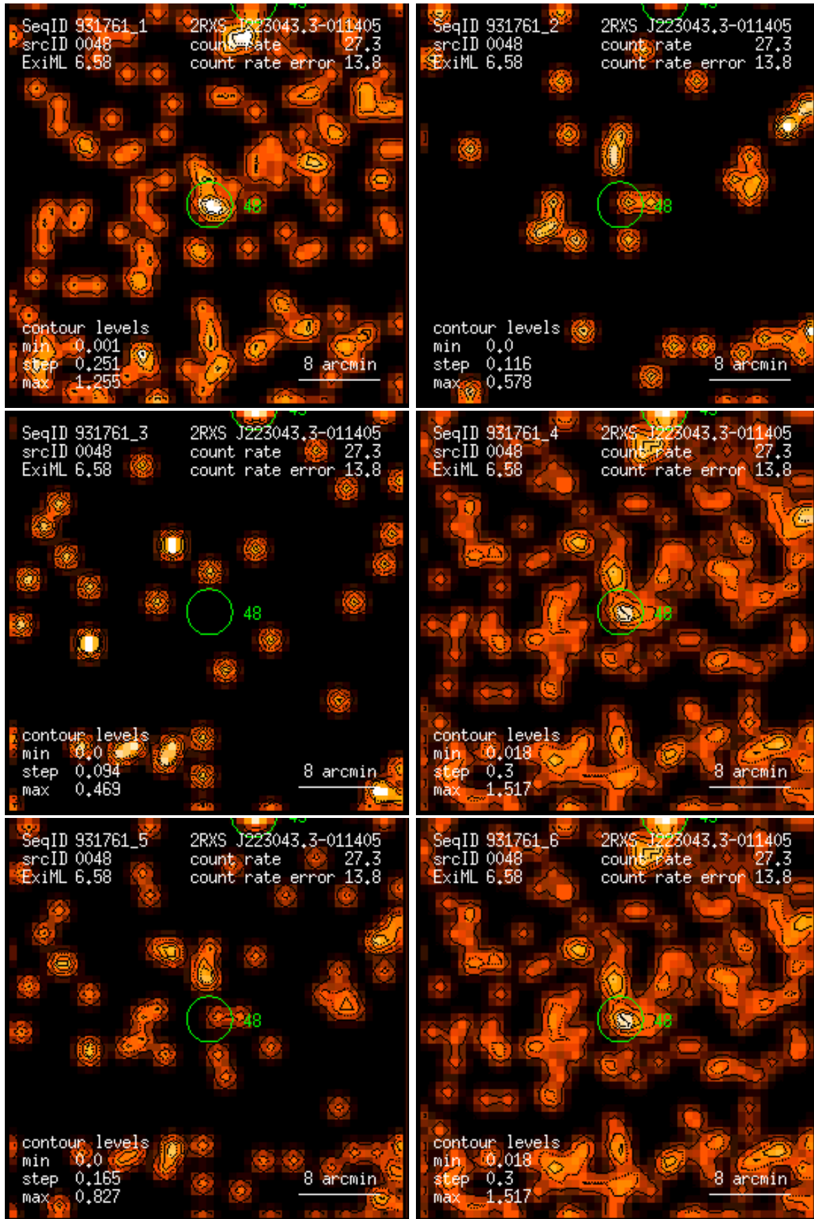
Figure 48: RASS 931761: detection 0048: band rate images, Gaussian filter: (1) PSPC channels 11 – 41, (2) 52 – 90, (3) 91 – 201, (4) 11 – 235, (5) 52 – 201, (6) 11 – 201. Broad band rates in counts/ks. Band rate contour levels in counts/ks/arcmin 2 .
