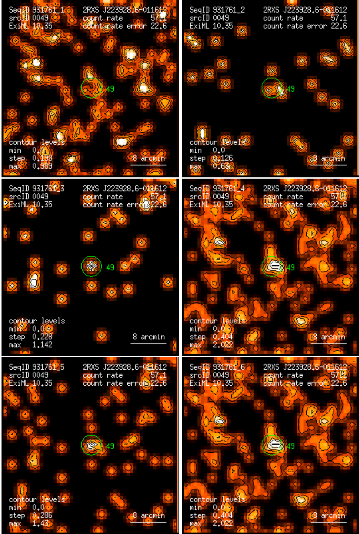
Figure 49: RASS 931761: detection 0049: band rate images, Gaussian filter: (1) PSPC channels 11 – 41, (2) 52 – 90, (3) 91 – 201, (4) 11 – 235, (5) 52 – 201, (6) 11 – 201. Broad band rates in counts/ks. Band rate contour levels in counts/ks/arcmin 2 .
