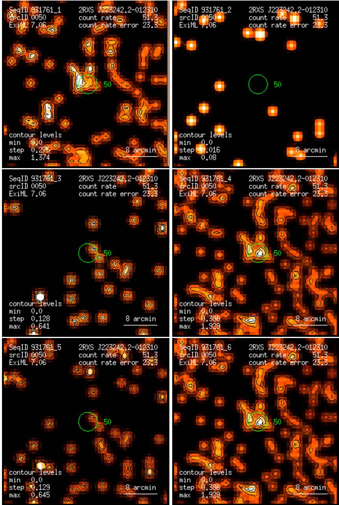
Figure 50: RASS 931761: detection 0050: band rate images, Gaussian filter: (1) PSPC channels 11 – 41, (2) 52 – 90, (3) 91 – 201, (4) 11 – 235, (5) 52 – 201, (6) 11 – 201. Broad band rates in counts/ks. Band rate contour levels in counts/ks/arcmin 2 .
