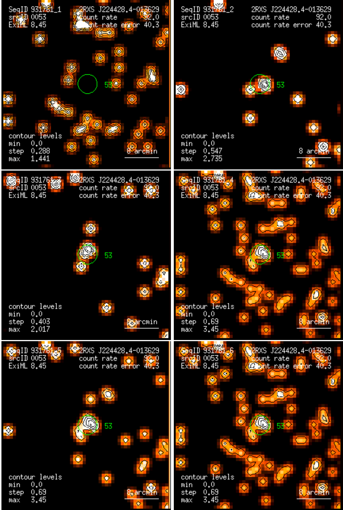
Figure 53: RASS 931761: detection 0053: band rate images, Gaussian filter: (1) PSPC channels 11 – 41, (2) 52 – 90, (3) 91 – 201, (4) 11 – 235, (5) 52 – 201, (6) 11 – 201. Broad band rates in counts/ks. Band rate contour levels in counts/ks/arcmin 2 .
