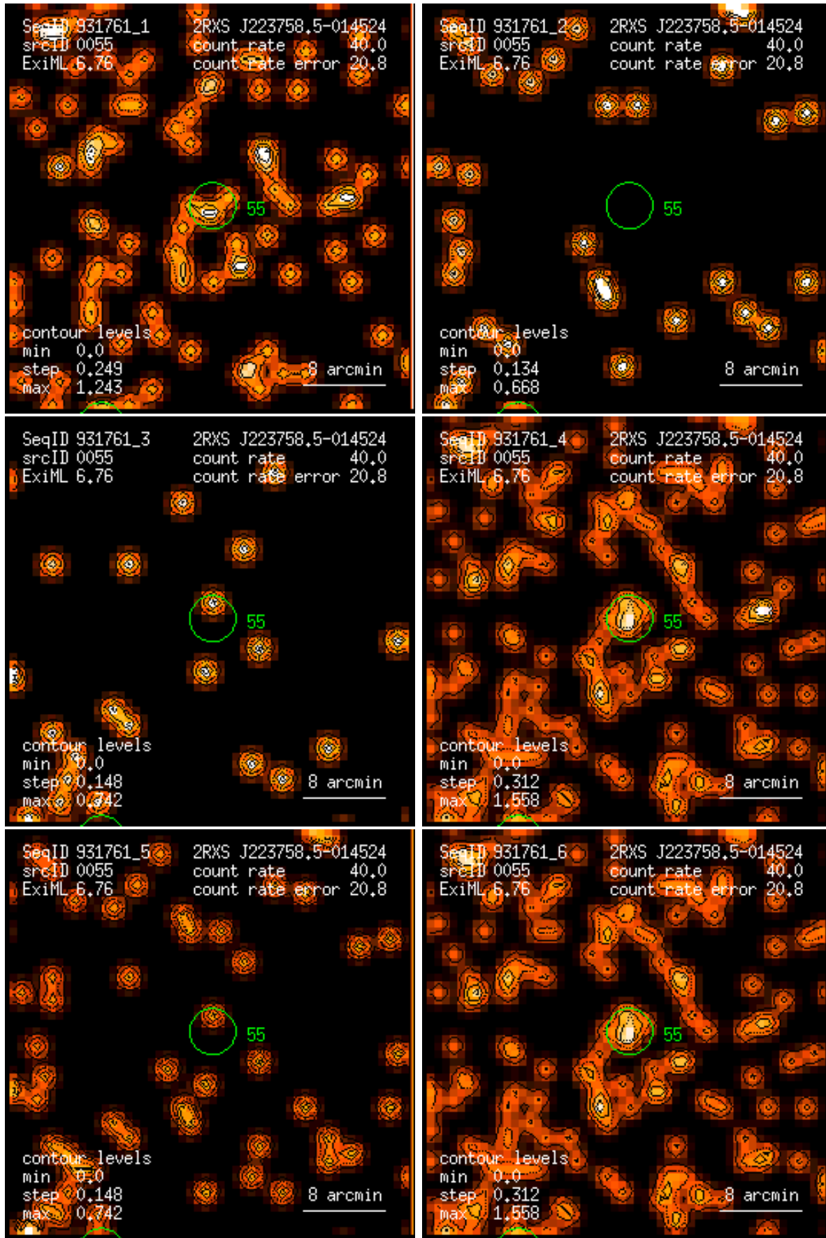
Figure 55: RASS 931761: detection 0055: band rate images, Gaussian filter: (1) PSPC channels 11 – 41, (2) 52 – 90, (3) 91 – 201, (4) 11 – 235, (5) 52 – 201, (6) 11 – 201. Broad band rates in counts/ks. Band rate contour levels in counts/ks/arcmin 2 .
