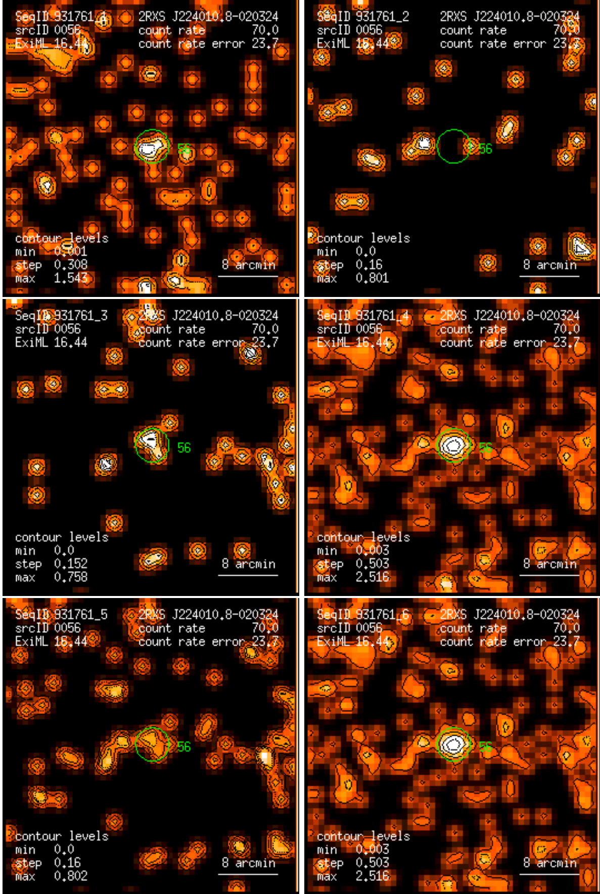
Figure 56: RASS 931761: detection 0056: band rate images, Gaussian filter: (1) PSPC channels 11 – 41, (2) 52 – 90, (3) 91 – 201, (4) 11 – 235, (5) 52 – 201, (6) 11 – 201. Broad band rates in counts/ks. Band rate contour levels in counts/ks/arcmin 2 .
