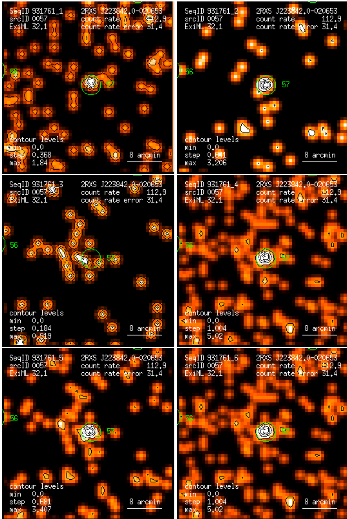
Figure 57: RASS 931761: detection 0057: band rate images, Gaussian filter: (1) PSPC channels 11 – 41, (2) 52 – 90, (3) 91 – 201, (4) 11 – 235, (5) 52 – 201, (6) 11 – 201. Broad band rates in counts/ks. Band rate contour levels in counts/ks/arcmin 2 .
