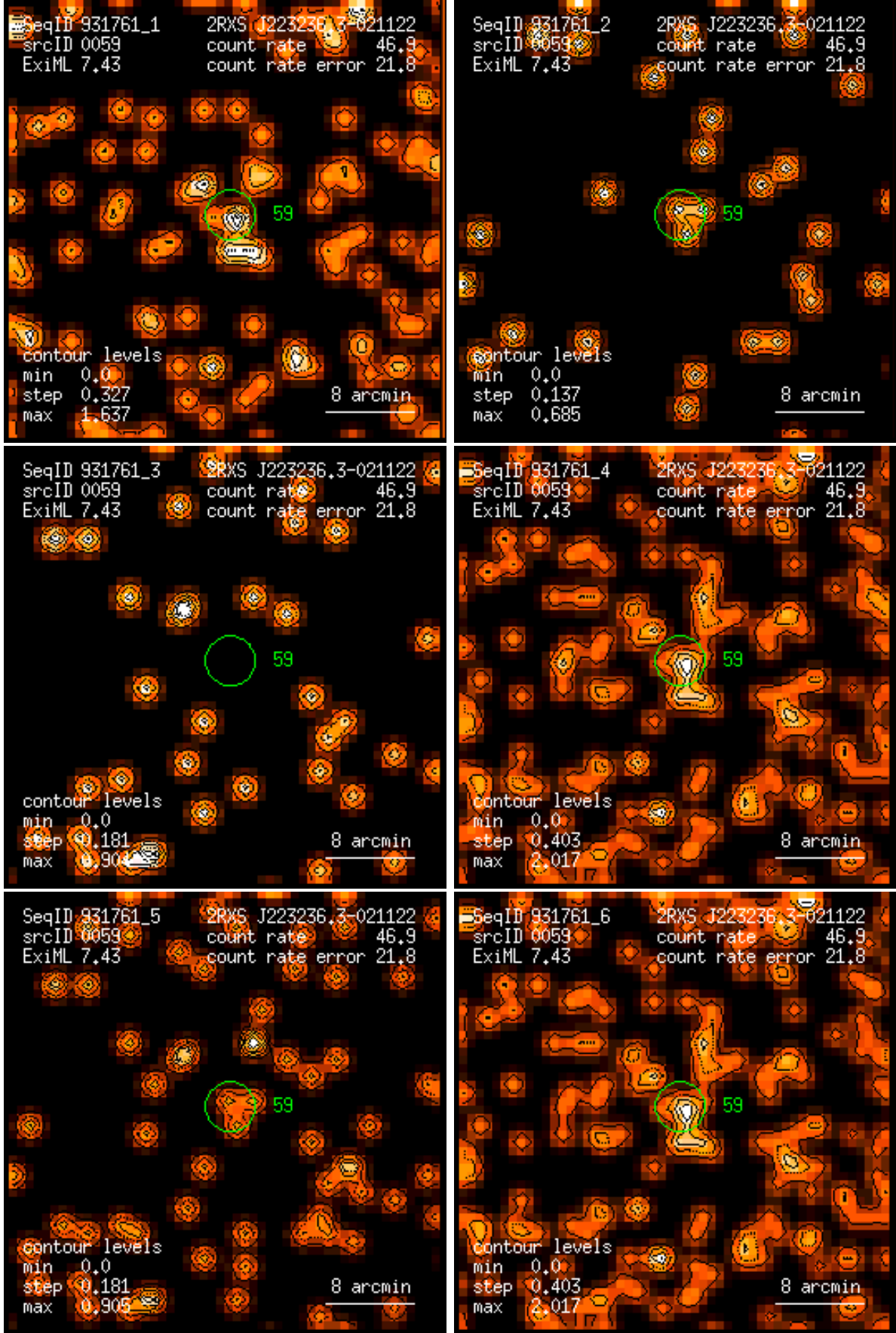
Figure 59: RASS 931761: detection 0059: band rate images, Gaussian filter: (1) PSPC channels 11 – 41, (2) 52 – 90, (3) 91 – 201, (4) 11 – 235, (5) 52 – 201, (6) 11 – 201. Broad band rates in counts/ks. Band rate contour levels in counts/ks/arcmin 2 .
