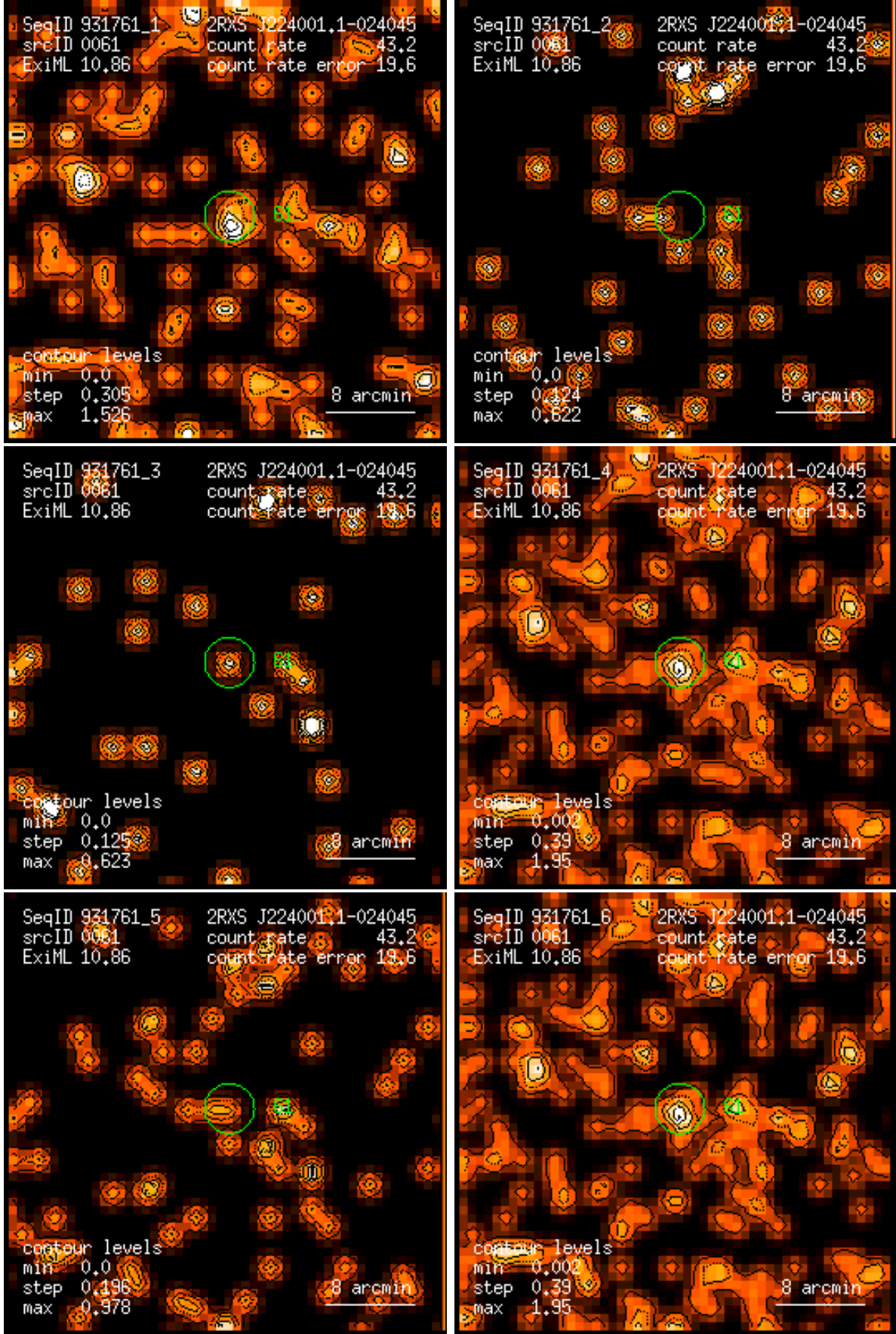
Figure 61: RASS 931761: detection 0061: band rate images, Gaussian filter: (1) PSPC channels 11 – 41, (2) 52 – 90, (3) 91 – 201, (4) 11 – 235, (5) 52 – 201, (6) 11 – 201. Broad band rates in counts/ks. Band rate contour levels in counts/ks/arcmin 2 .
