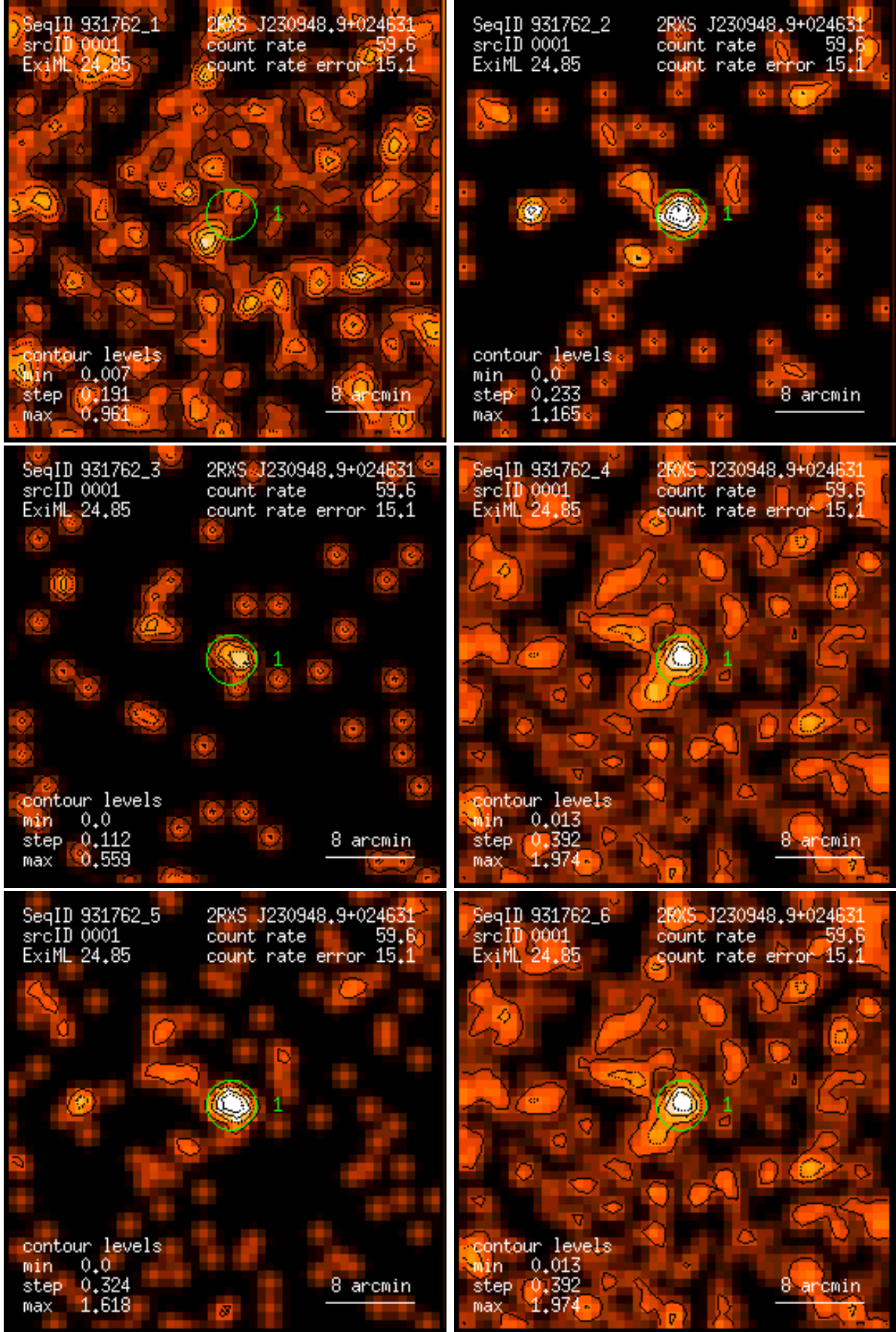
Figure 1: RASS 931762: detection 0001: band rate images, Gaussian filter: (1) PSPC channels 11 – 41, (2) 52 – 90, (3) 91 – 201, (4) 11 – 235, (5) 52 – 201, (6) 11 – 201. Broad band rates in counts/ks. Band rate contour levels in counts/ks/arcmin 2 .
