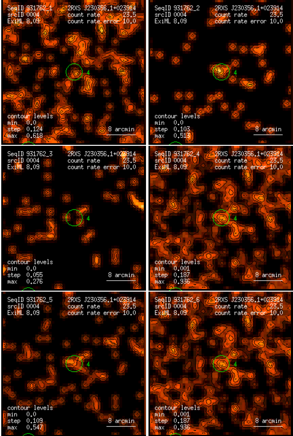
Figure 4: RASS 931762: detection 0004: band rate images, Gaussian filter: (1) PSPC channels 11 – 41, (2) 52 – 90, (3) 91 – 201, (4) 11 – 235, (5) 52 – 201, (6) 11 – 201. Broad band rates in counts/ks. Band rate contour levels in counts/ks/arcmin 2 .
