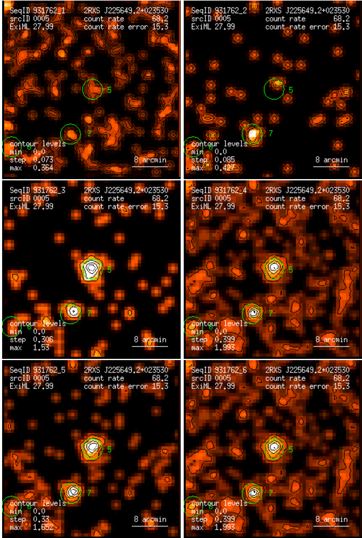
Figure 5: RASS 931762: detection 0005: band rate images, Gaussian filter: (1) PSPC channels 11 – 41, (2) 52 – 90, (3) 91 – 201, (4) 11 – 235, (5) 52 – 201, (6) 11 – 201. Broad band rates in counts/ks. Band rate contour levels in counts/ks/arcmin 2 .
