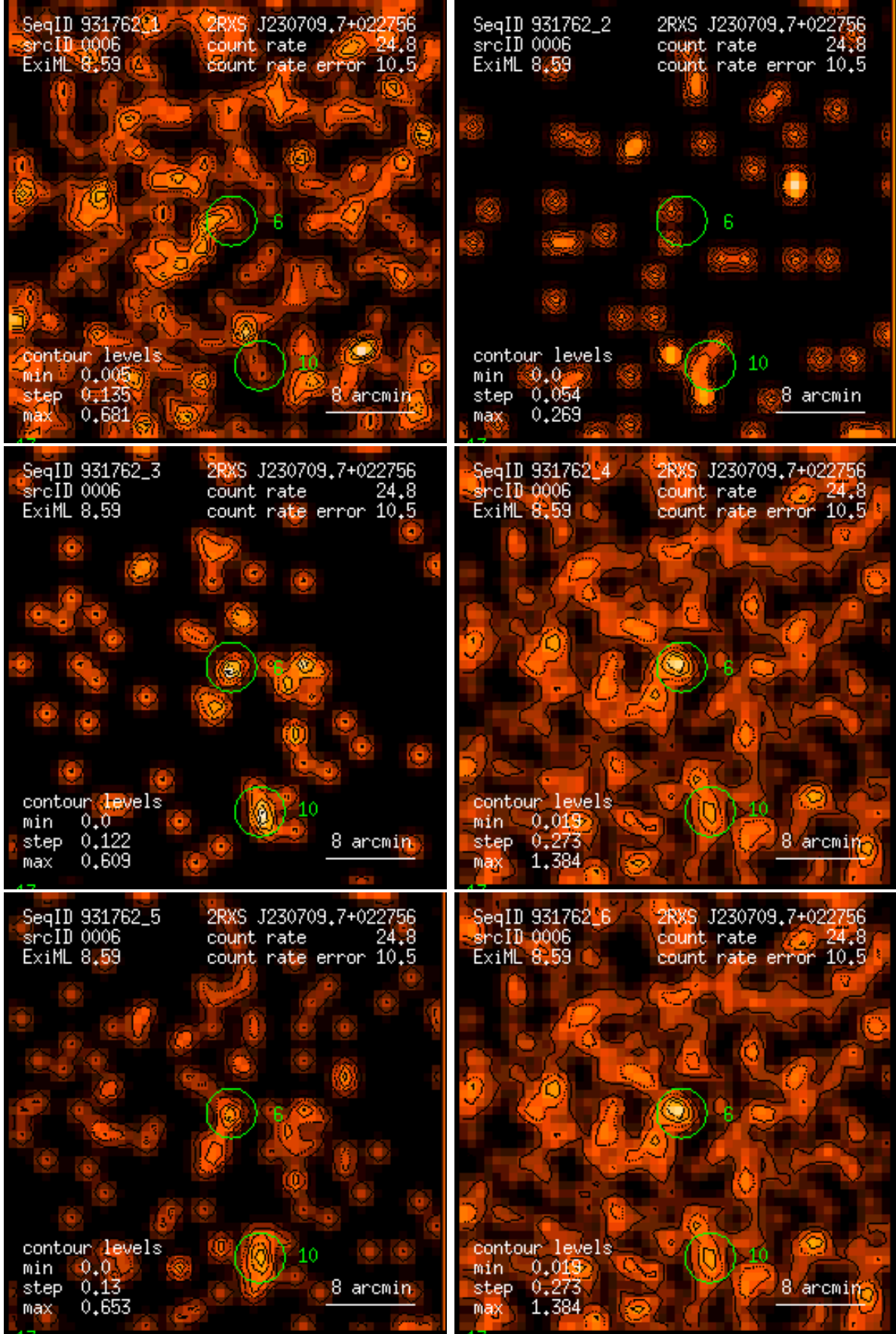
Figure 6: RASS 931762: detection 0006: band rate images, Gaussian filter: (1) PSPC channels 11 – 41, (2) 52 – 90, (3) 91 – 201, (4) 11 – 235, (5) 52 – 201, (6) 11 – 201. Broad band rates in counts/ks. Band rate contour levels in counts/ks/arcmin 2 .
