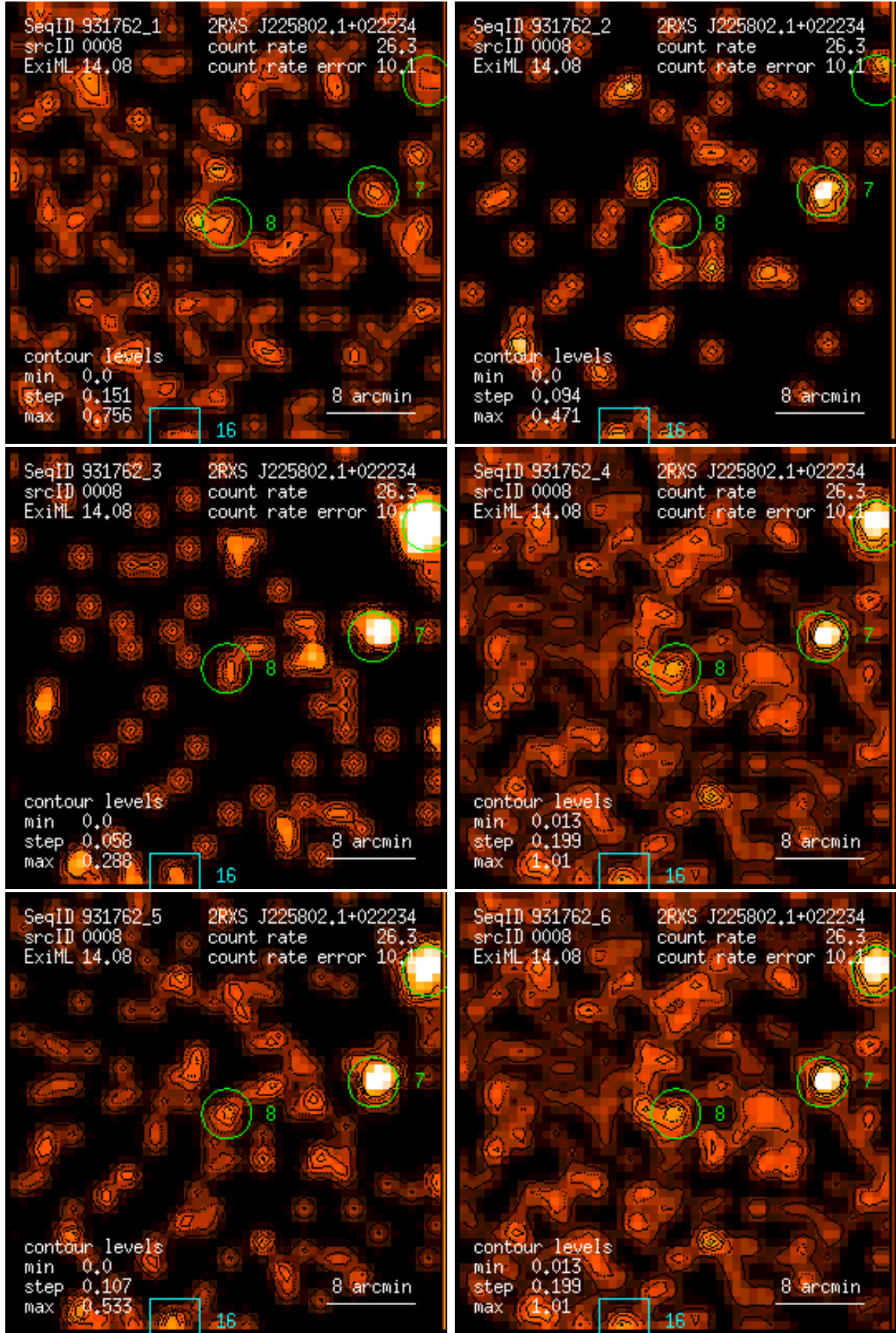
Figure 8: RASS 931762: detection 0008: band rate images, Gaussian filter: (1) PSPC channels 11 – 41, (2) 52 – 90, (3) 91 – 201, (4) 11 – 235, (5) 52 – 201, (6) 11 – 201. Broad band rates in counts/ks. Band rate contour levels in counts/ks/arcmin 2 .
