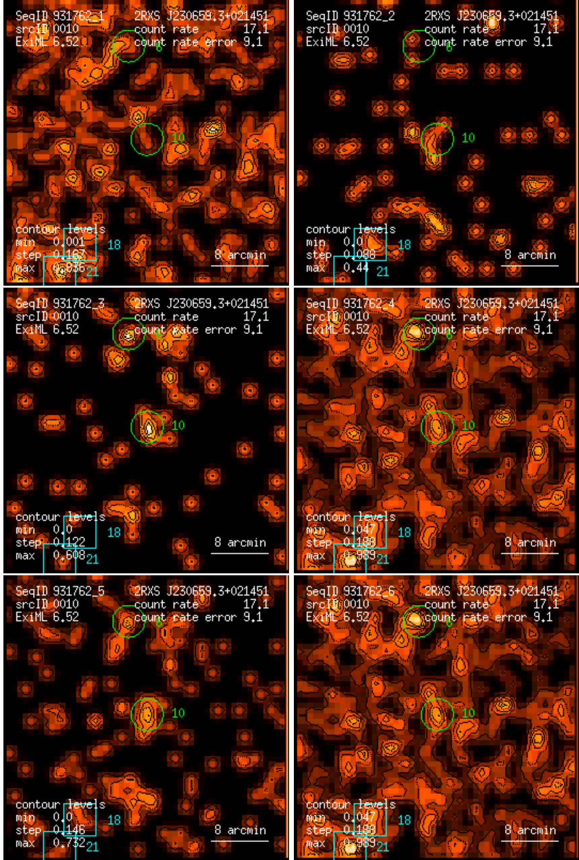
Figure 10: RASS 931762: detection 0010: band rate images, Gaussian filter: (1) PSPC channels 11 – 41, (2) 52 – 90, (3) 91 – 201, (4) 11 – 235, (5) 52 – 201, (6) 11 – 201. Broad band rates in counts/ks. Band rate contour levels in counts/ks/arcmin 2 .
