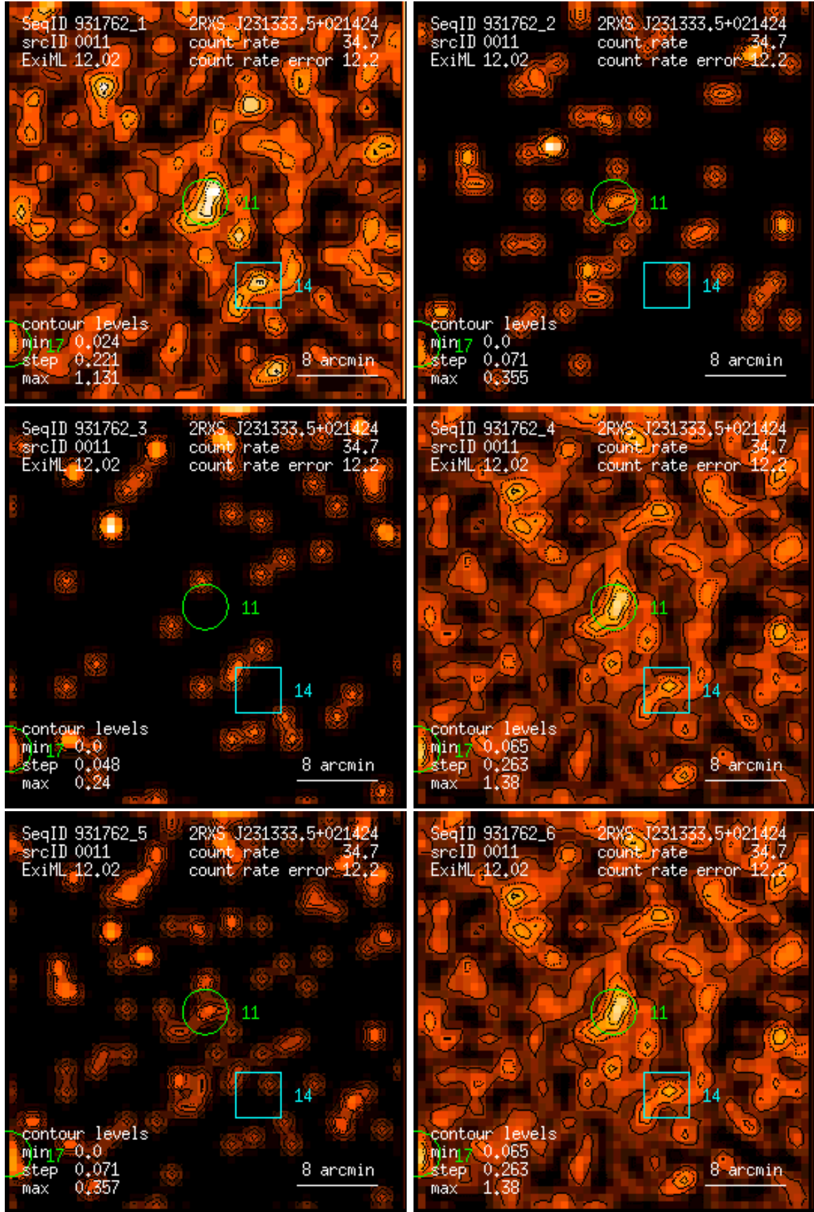
Figure 11: RASS 931762: detection 0011: band rate images, Gaussian filter: (1) PSPC channels 11 – 41, (2) 52 – 90, (3) 91 – 201, (4) 11 – 235, (5) 52 – 201, (6) 11 – 201. Broad band rates in counts/ks. Band rate contour levels in counts/ks/arcmin 2 .
