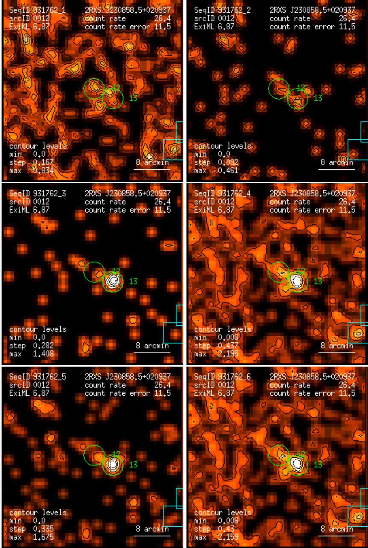
Figure 12: RASS 931762: detection 0012: band rate images, Gaussian filter: (1) PSPC channels 11 – 41, (2) 52 – 90, (3) 91 – 201, (4) 11 – 235, (5) 52 – 201, (6) 11 – 201. Broad band rates in counts/ks. Band rate contour levels in counts/ks/arcmin 2 .
