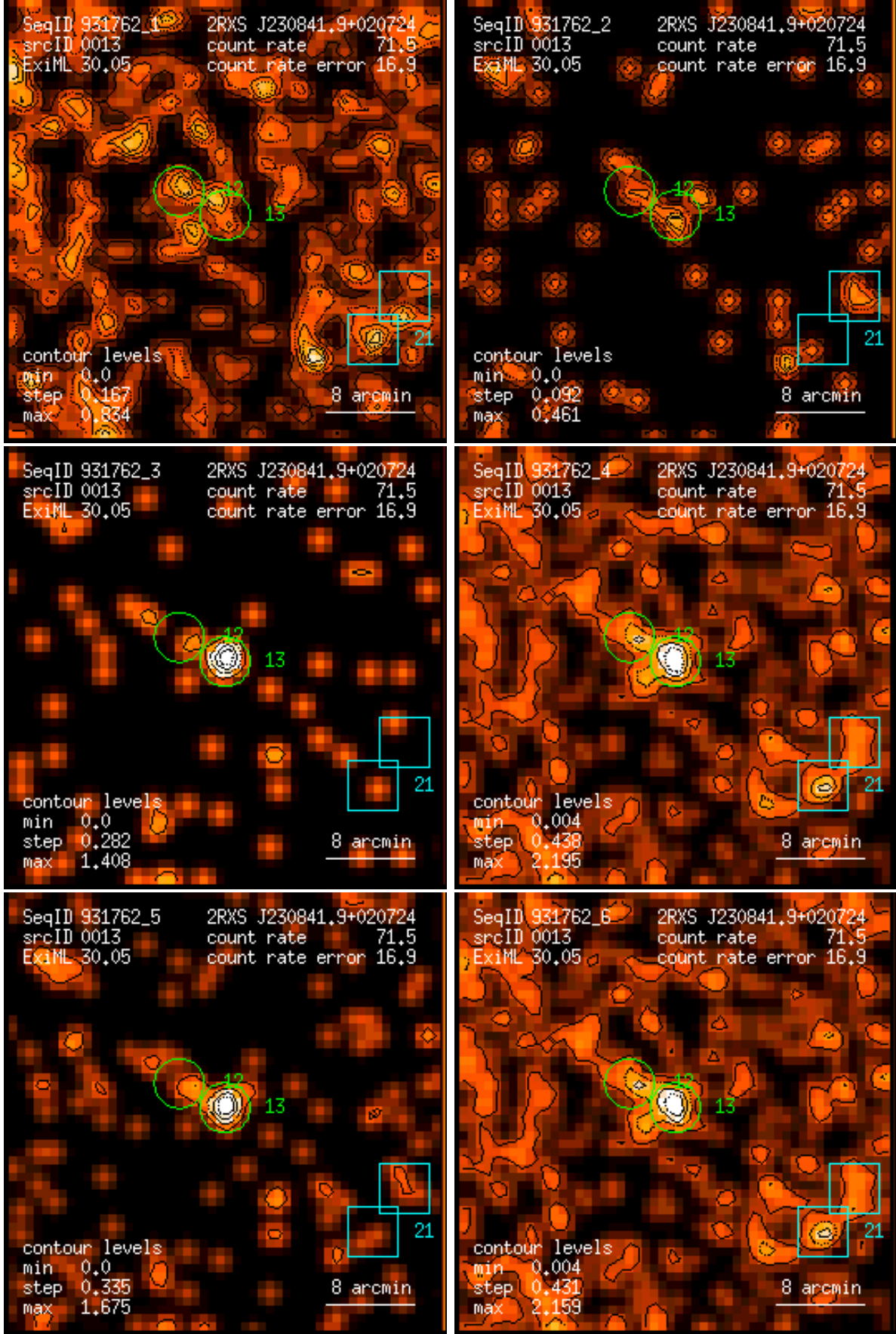
Figure 13: RASS 931762: detection 0013: band rate images, Gaussian filter: (1) PSPC channels 11 – 41, (2) 52 – 90, (3) 91 – 201, (4) 11 – 235, (5) 52 – 201, (6) 11 – 201. Broad band rates in counts/ks. Band rate contour levels in counts/ks/arcmin 2 .
