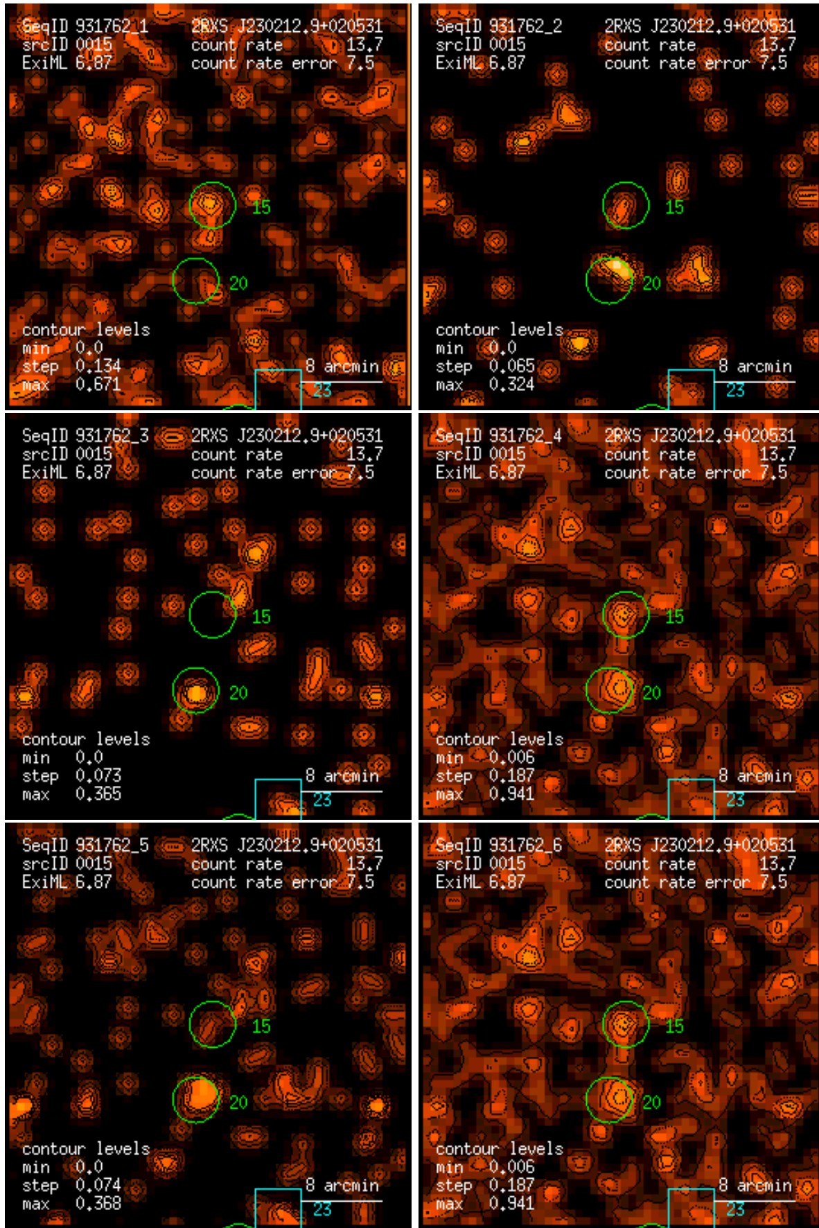
Figure 15: RASS 931762: detection 0015: band rate images, Gaussian filter: (1) PSPC channels 11 – 41, (2) 52 – 90, (3) 91 – 201, (4) 11 – 235, (5) 52 – 201, (6) 11 – 201. Broad band rates in counts/ks. Band rate contour levels in counts/ks/arcmin 2 .
