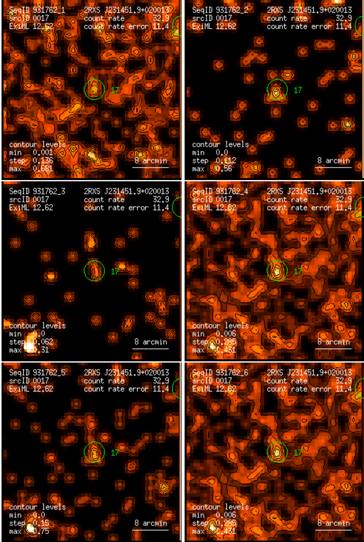
Figure 17: RASS 931762: detection 0017: band rate images, Gaussian filter: (1) PSPC channels 11 – 41, (2) 52 – 90, (3) 91 – 201, (4) 11 – 235, (5) 52 – 201, (6) 11 – 201. Broad band rates in counts/ks. Band rate contour levels in counts/ks/arcmin 2 .
