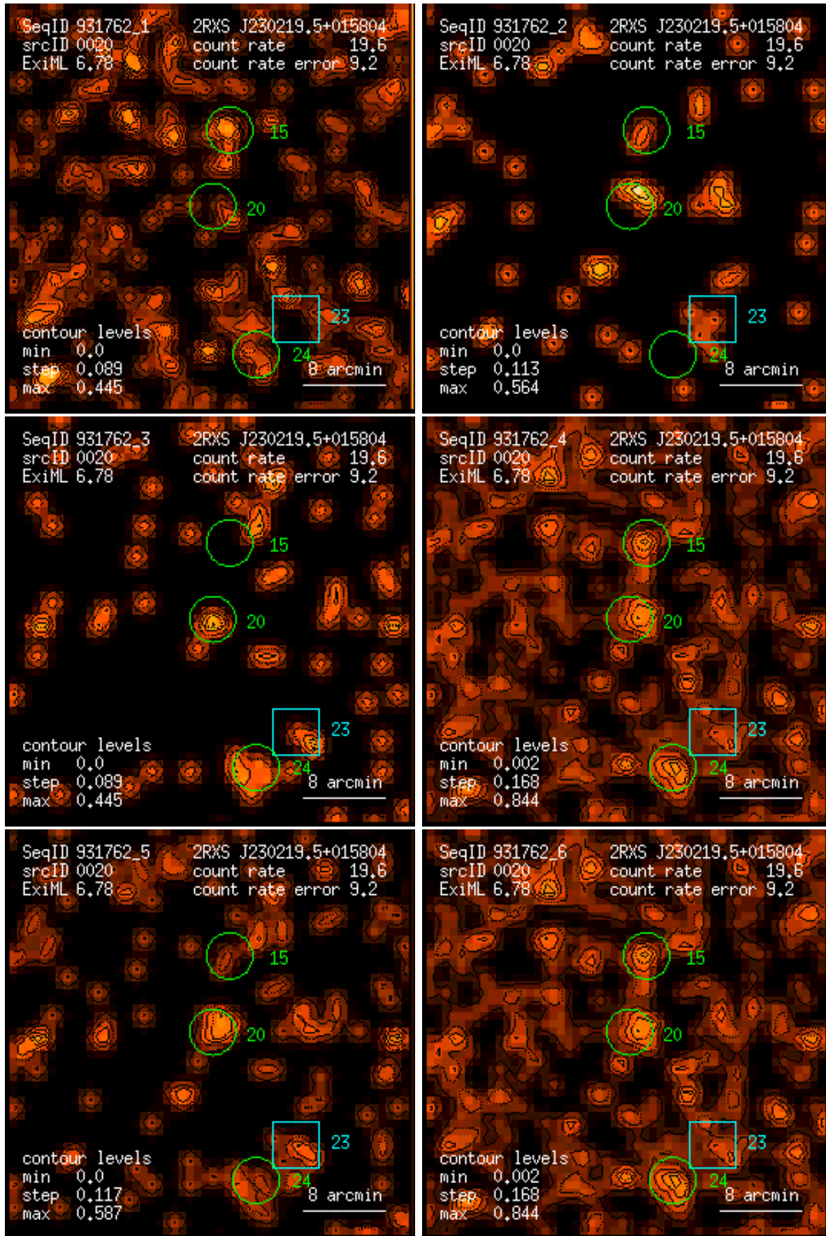
Figure 20: RASS 931762: detection 0020: band rate images, Gaussian filter: (1) PSPC channels 11 – 41, (2) 52 – 90, (3) 91 – 201, (4) 11 – 235, (5) 52 – 201, (6) 11 – 201. Broad band rates in counts/ks. Band rate contour levels in counts/ks/arcmin 2 .
