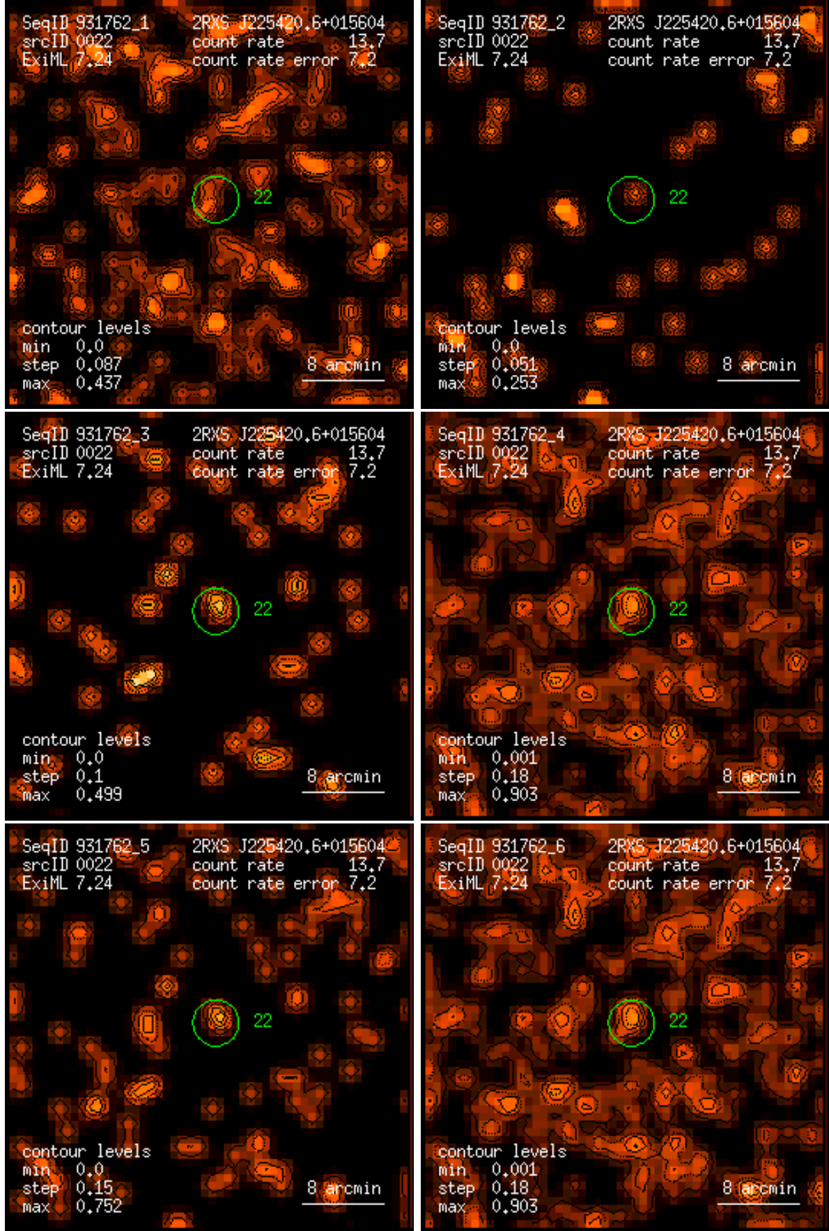
Figure 22: RASS 931762: detection 0022: band rate images, Gaussian filter: (1) PSPC channels 11 – 41, (2) 52 – 90, (3) 91 – 201, (4) 11 – 235, (5) 52 – 201, (6) 11 – 201. Broad band rates in counts/ks. Band rate contour levels in counts/ks/arcmin 2 .
