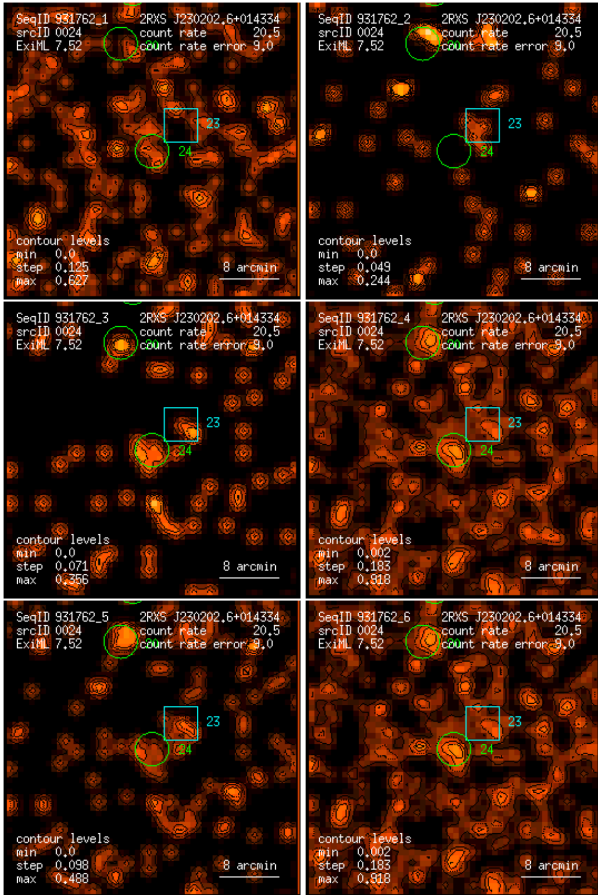
Figure 24: RASS 931762: detection 0024: band rate images, Gaussian filter: (1) PSPC channels 11 – 41, (2) 52 – 90, (3) 91 – 201, (4) 11 – 235, (5) 52 – 201, (6) 11 – 201. Broad band rates in counts/ks. Band rate contour levels in counts/ks/arcmin 2 .
