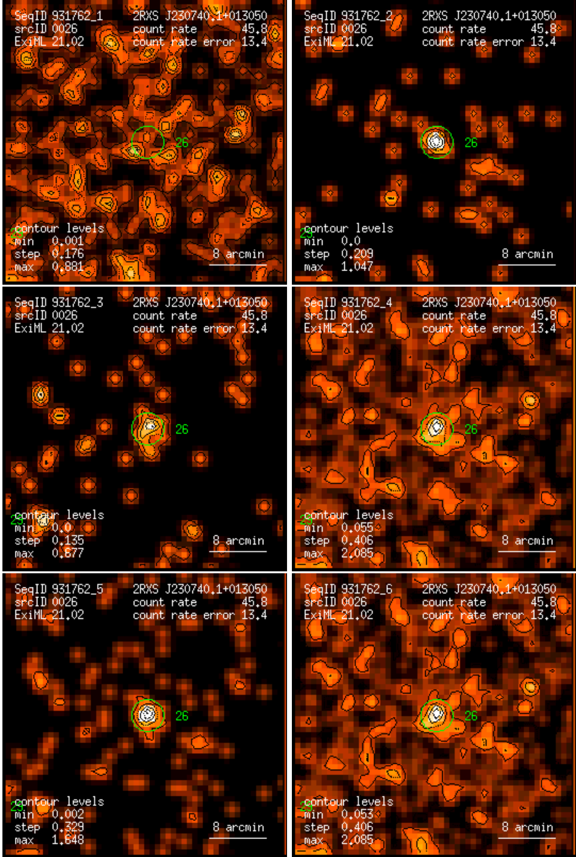
Figure 26: RASS 931762: detection 0026: band rate images, Gaussian filter: (1) PSPC channels 11 – 41, (2) 52 – 90, (3) 91 – 201, (4) 11 – 235, (5) 52 – 201, (6) 11 – 201. Broad band rates in counts/ks. Band rate contour levels in counts/ks/arcmin 2 .
