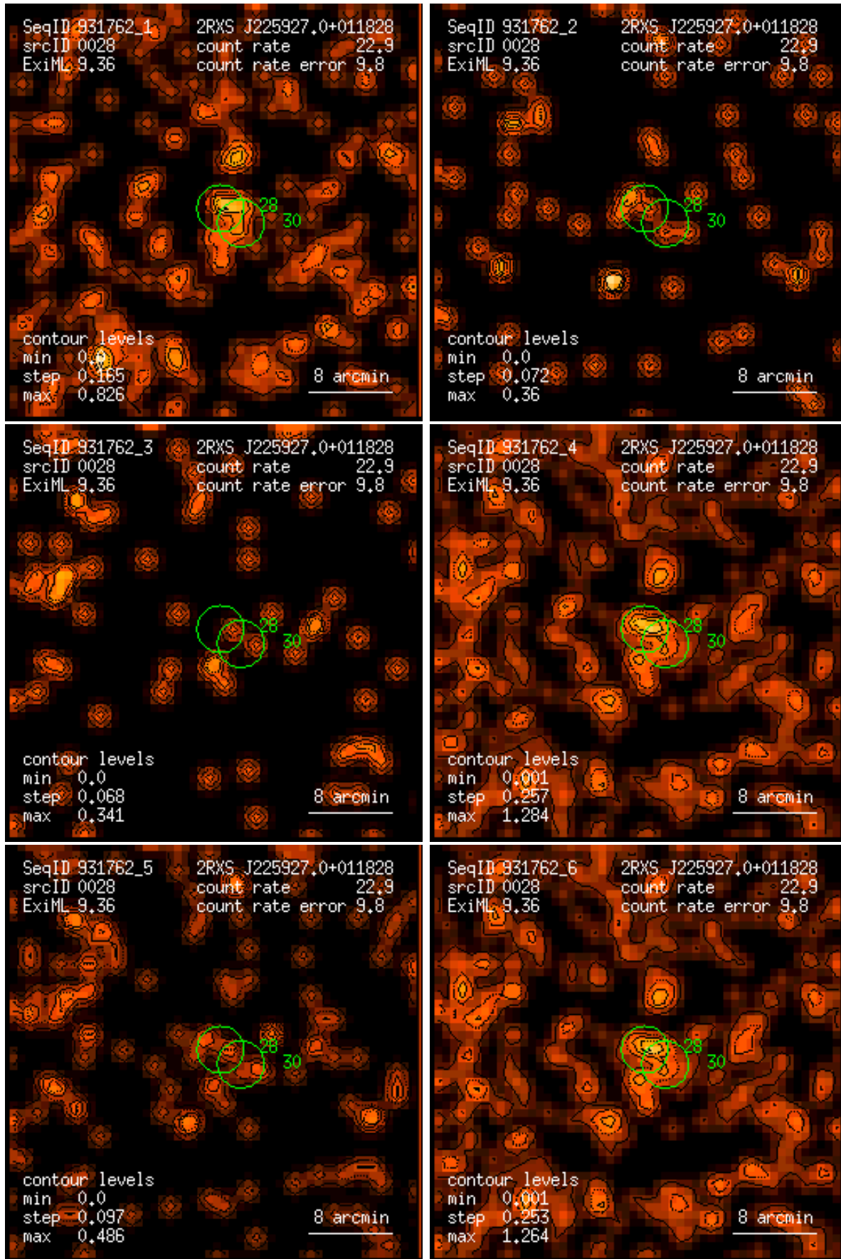
Figure 28: RASS 931762: detection 0028: band rate images, Gaussian filter: (1) PSPC channels 11 – 41, (2) 52 – 90, (3) 91 – 201, (4) 11 – 235, (5) 52 – 201, (6) 11 – 201. Broad band rates in counts/ks. Band rate contour levels in counts/ks/arcmin 2 .
