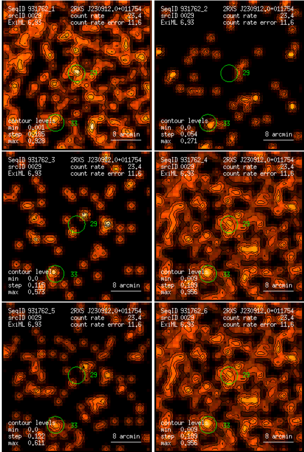
Figure 29: RASS 931762: detection 0029: band rate images, Gaussian filter: (1) PSPC channels 11 – 41, (2) 52 – 90, (3) 91 – 201, (4) 11 – 235, (5) 52 – 201, (6) 11 – 201. Broad band rates in counts/ks. Band rate contour levels in counts/ks/arcmin 2 .
