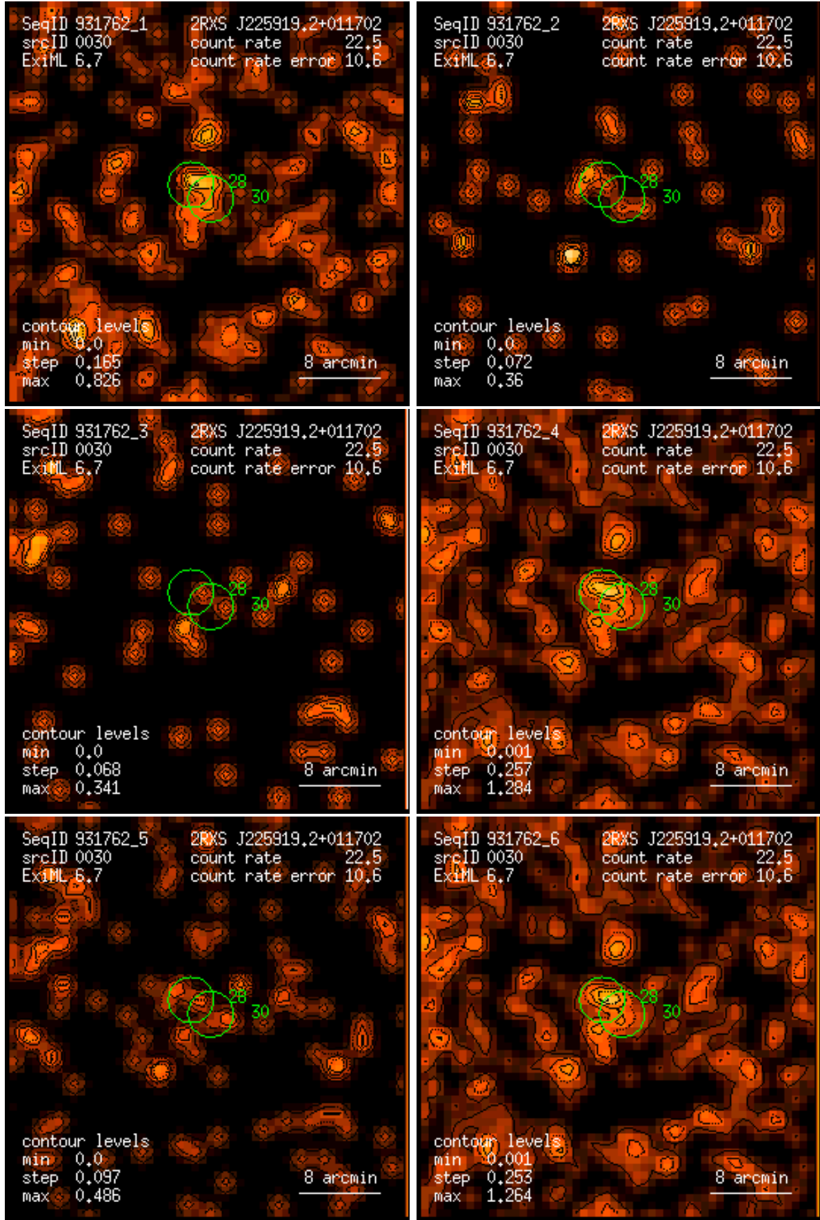
Figure 30: RASS 931762: detection 0030: band rate images, Gaussian filter: (1) PSPC channels 11 – 41, (2) 52 – 90, (3) 91 – 201, (4) 11 – 235, (5) 52 – 201, (6) 11 – 201. Broad band rates in counts/ks. Band rate contour levels in counts/ks/arcmin 2 .
