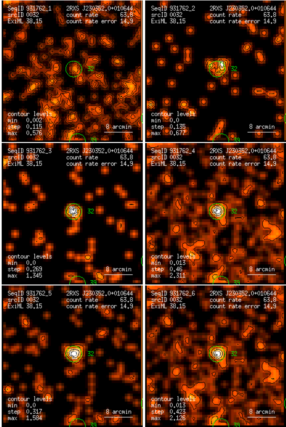
Figure 32: RASS 931762: detection 0032: band rate images, Gaussian filter: (1) PSPC channels 11 – 41, (2) 52 – 90, (3) 91 – 201, (4) 11 – 235, (5) 52 – 201, (6) 11 – 201. Broad band rates in counts/ks. Band rate contour levels in counts/ks/arcmin 2 .
