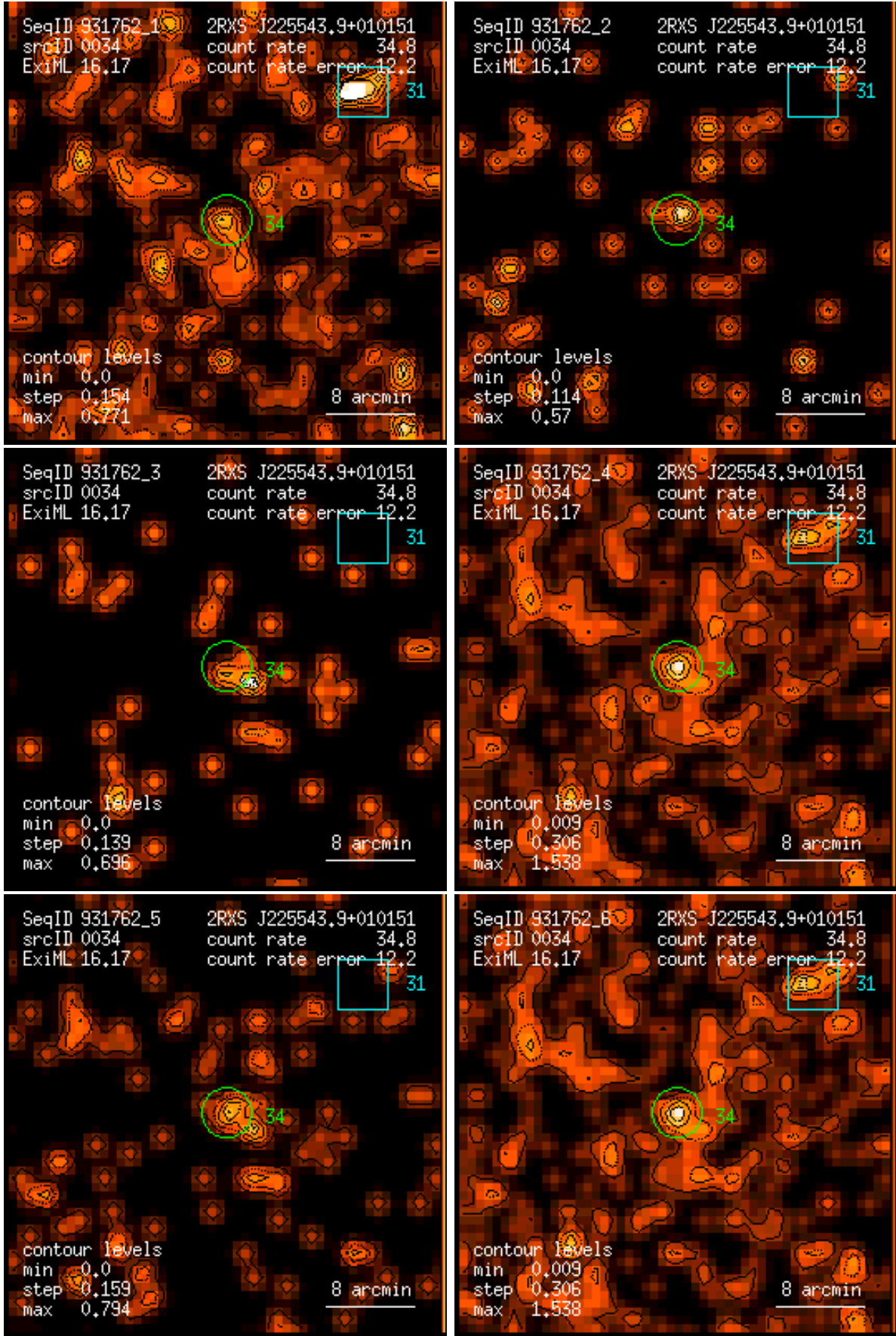
Figure 34: RASS 931762: detection 0034: band rate images, Gaussian filter: (1) PSPC channels 11 – 41, (2) 52 – 90, (3) 91 – 201, (4) 11 – 235, (5) 52 – 201, (6) 11 – 201. Broad band rates in counts/ks. Band rate contour levels in counts/ks/arcmin 2 .
