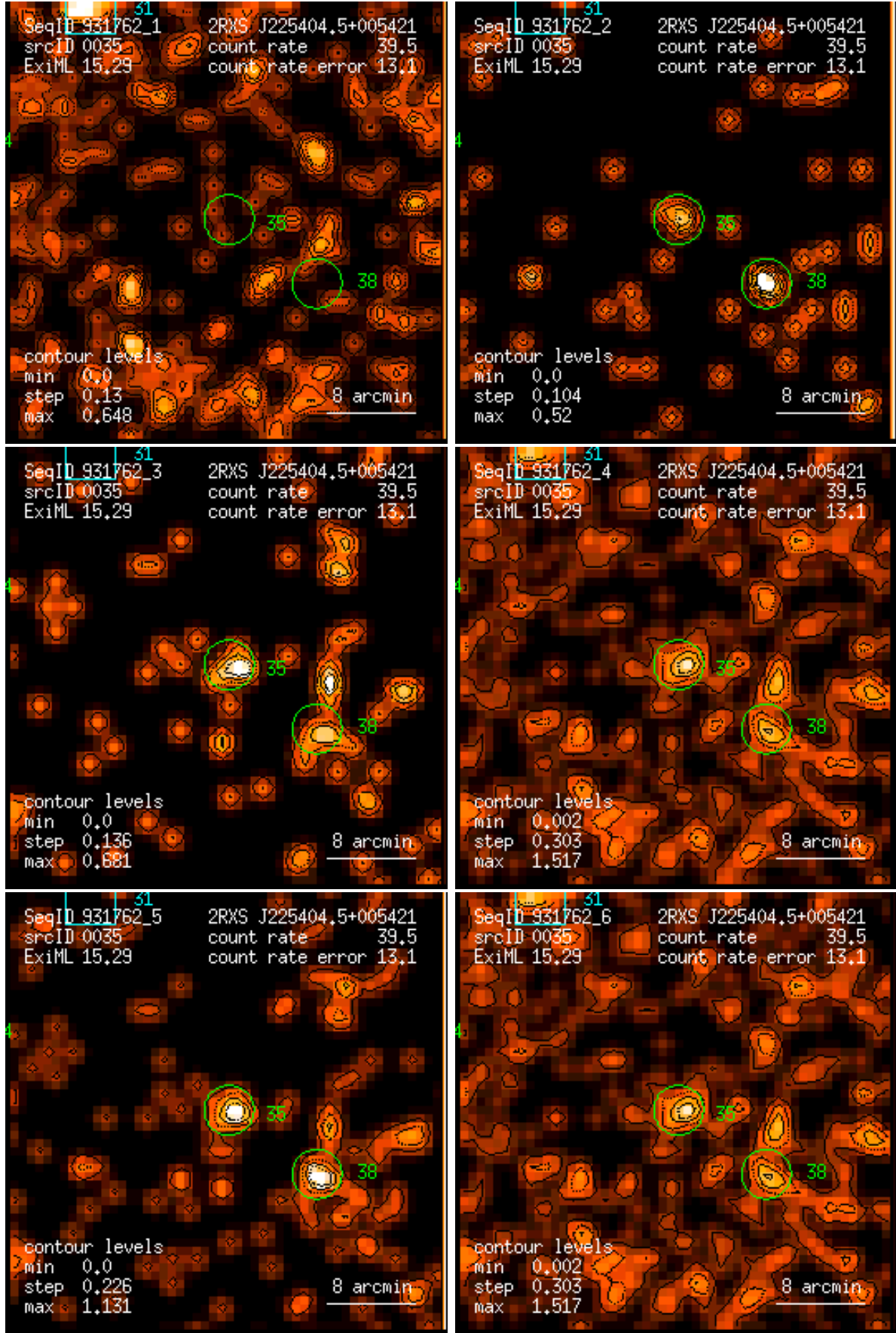
Figure 35: RASS 931762: detection 0035: band rate images, Gaussian filter: (1) PSPC channels 11 – 41, (2) 52 – 90, (3) 91 – 201, (4) 11 – 235, (5) 52 – 201, (6) 11 – 201. Broad band rates in counts/ks. Band rate contour levels in counts/ks/arcmin 2 .
